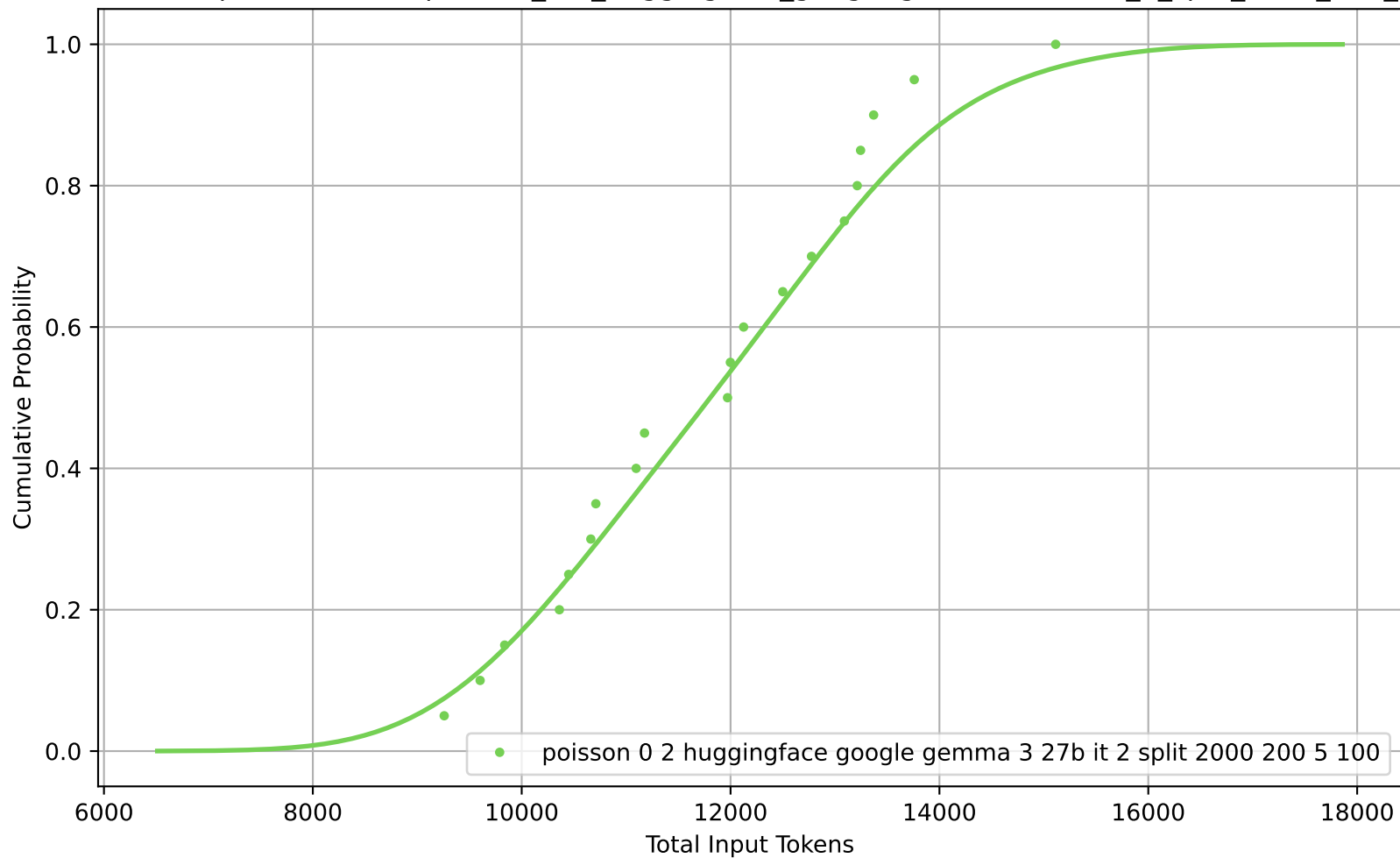
CDF of Total Input Tokens for poisson_0-2_huggingface_google-gemma-3-27b-it_2_split_2000_200_5_100
