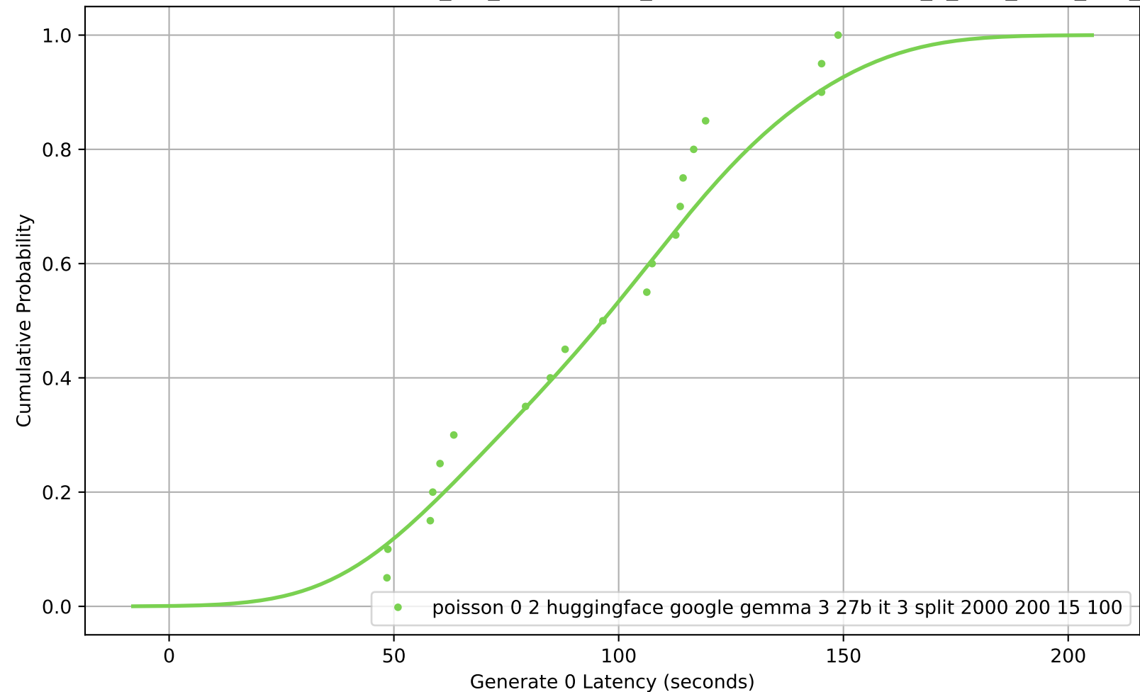
CDF of Generate 0 Latency for poisson_0-2_huggingface_google-gemma-3-27b-it_3_split_2000_200_15_100
