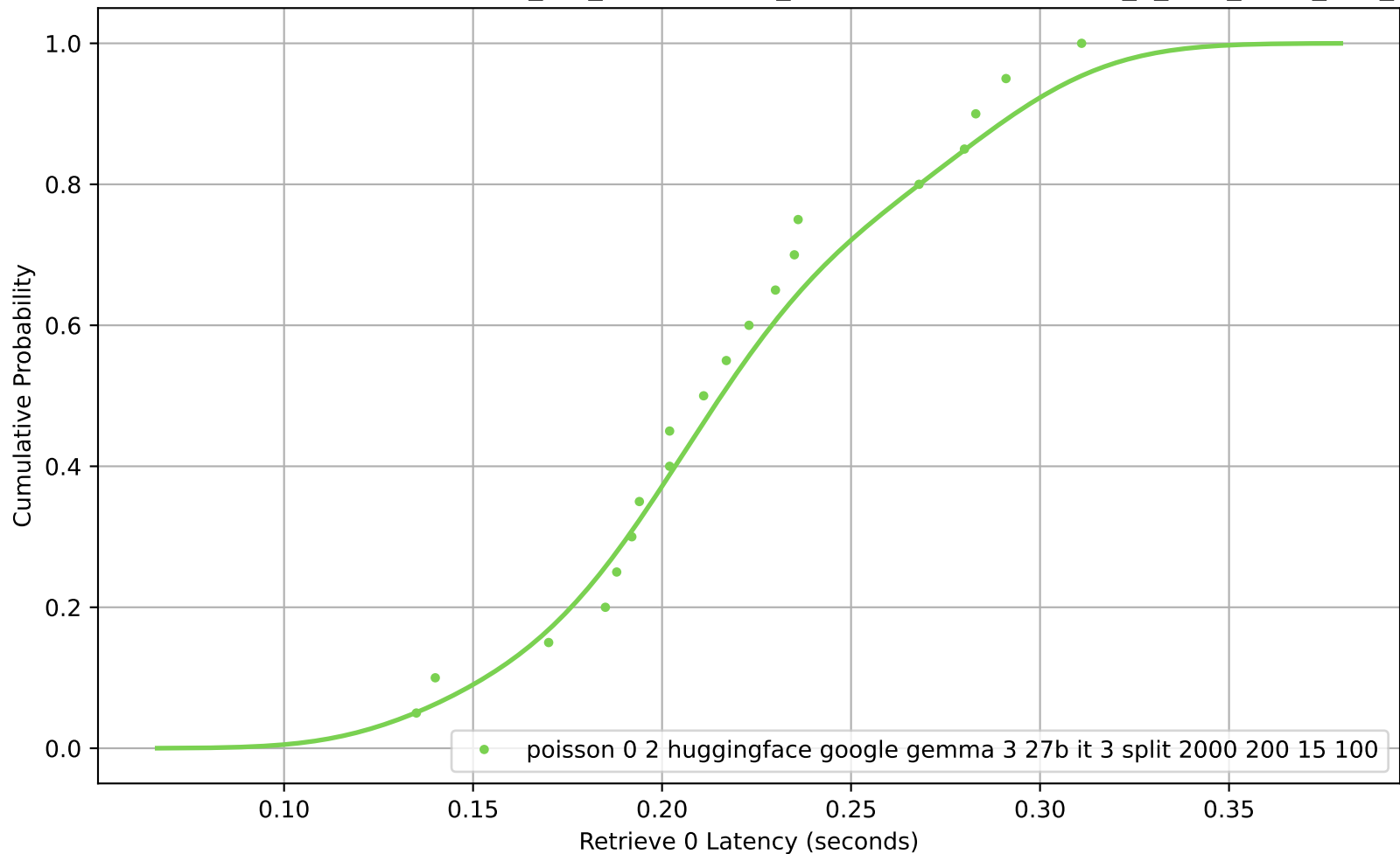
CDF of Retrieve 0 Latency for poisson_0-2_huggingface_google-gemma-3-27b-it_3_split_2000_200_15_100
