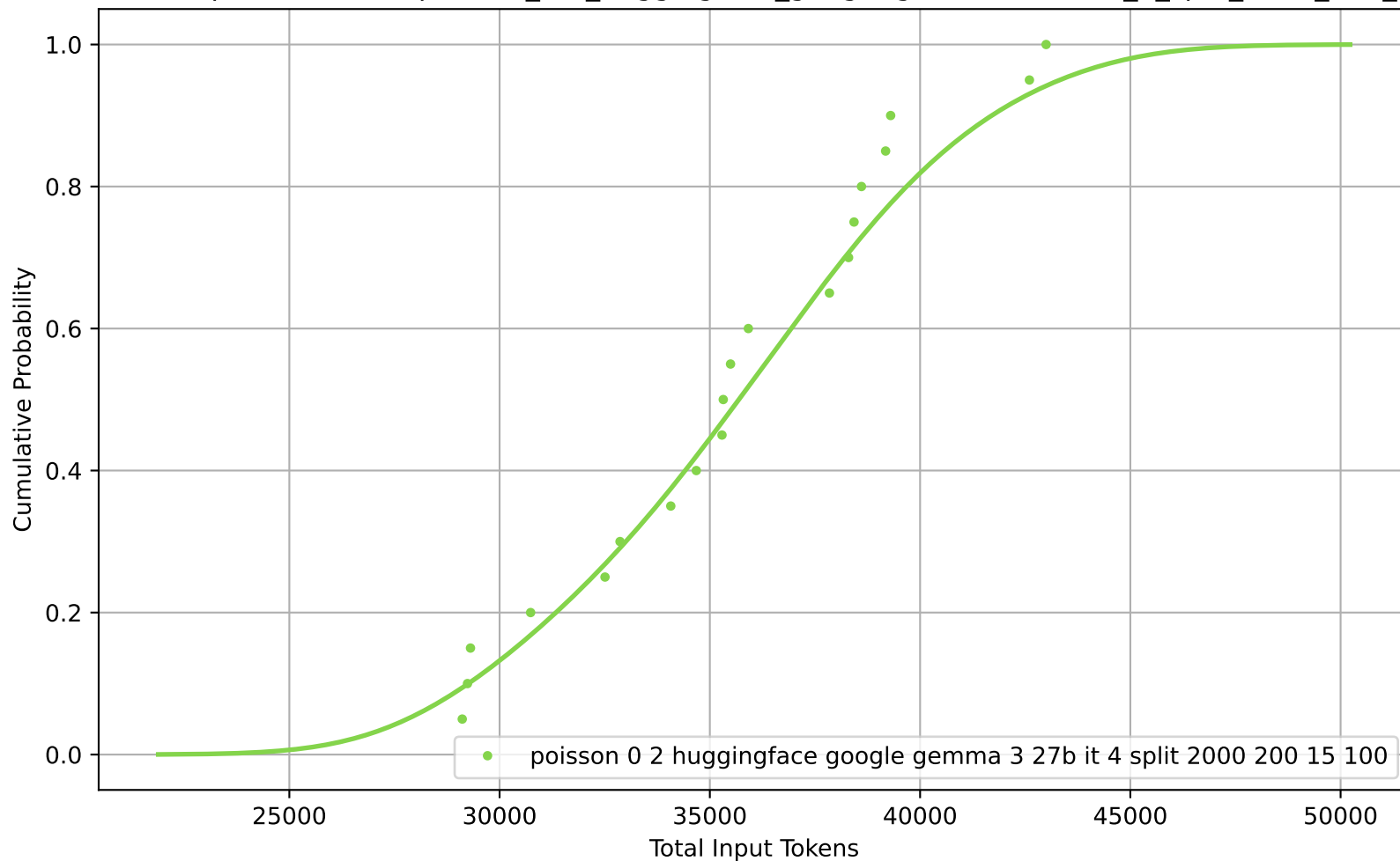
CDF of Total Input Tokens for poisson_0-2_huggingface_google-gemma-3-27b-it_4_split_2000_200_15_100
