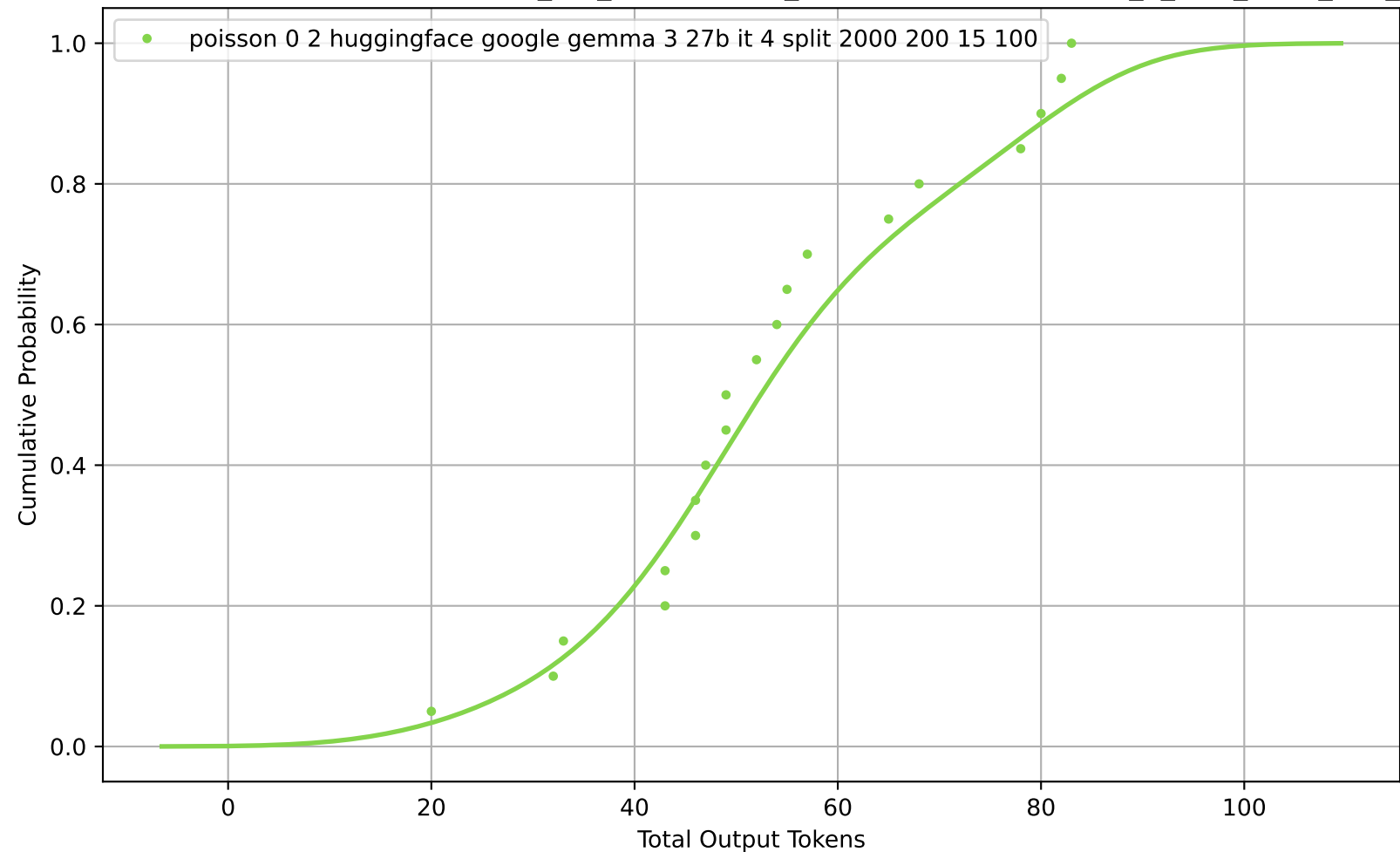
CDF of Total Output Tokens for poisson_0-2_huggingface_google-gemma-3-27b-it_4_split_2000_200_15_100
