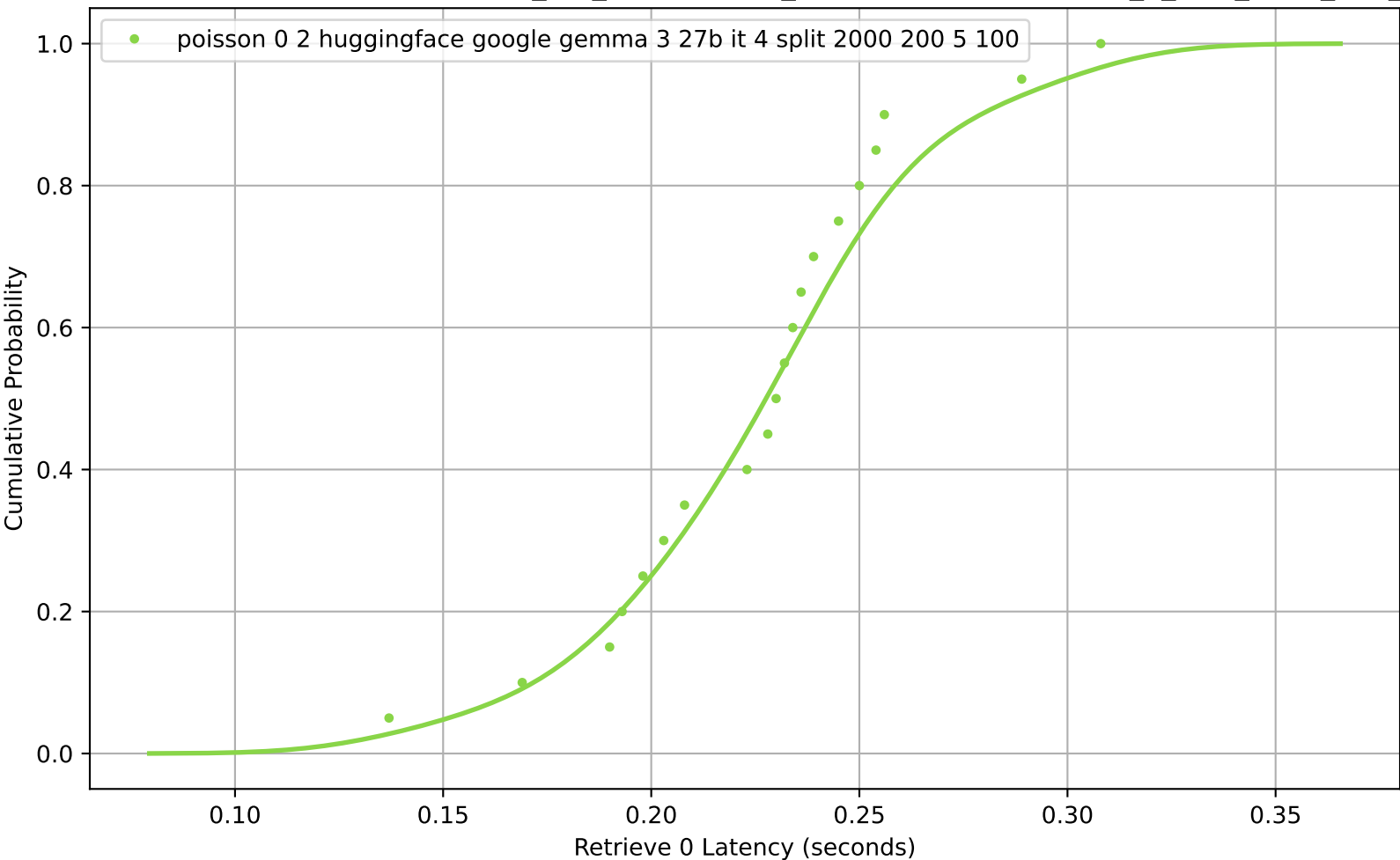
CDF of Retrieve 0 Latency for poisson_0-2_huggingface_google-gemma-3-27b-it_4_split_2000_200_5_100
