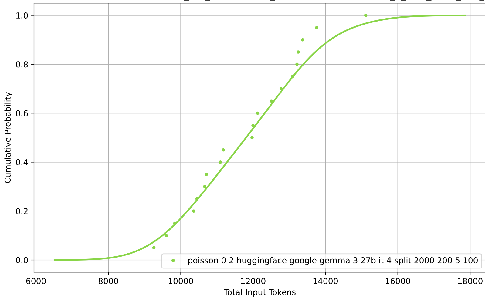
CDF of Total Input Tokens for poisson_0-2_huggingface_google-gemma-3-27b-it_4_split_2000_200_5_100
