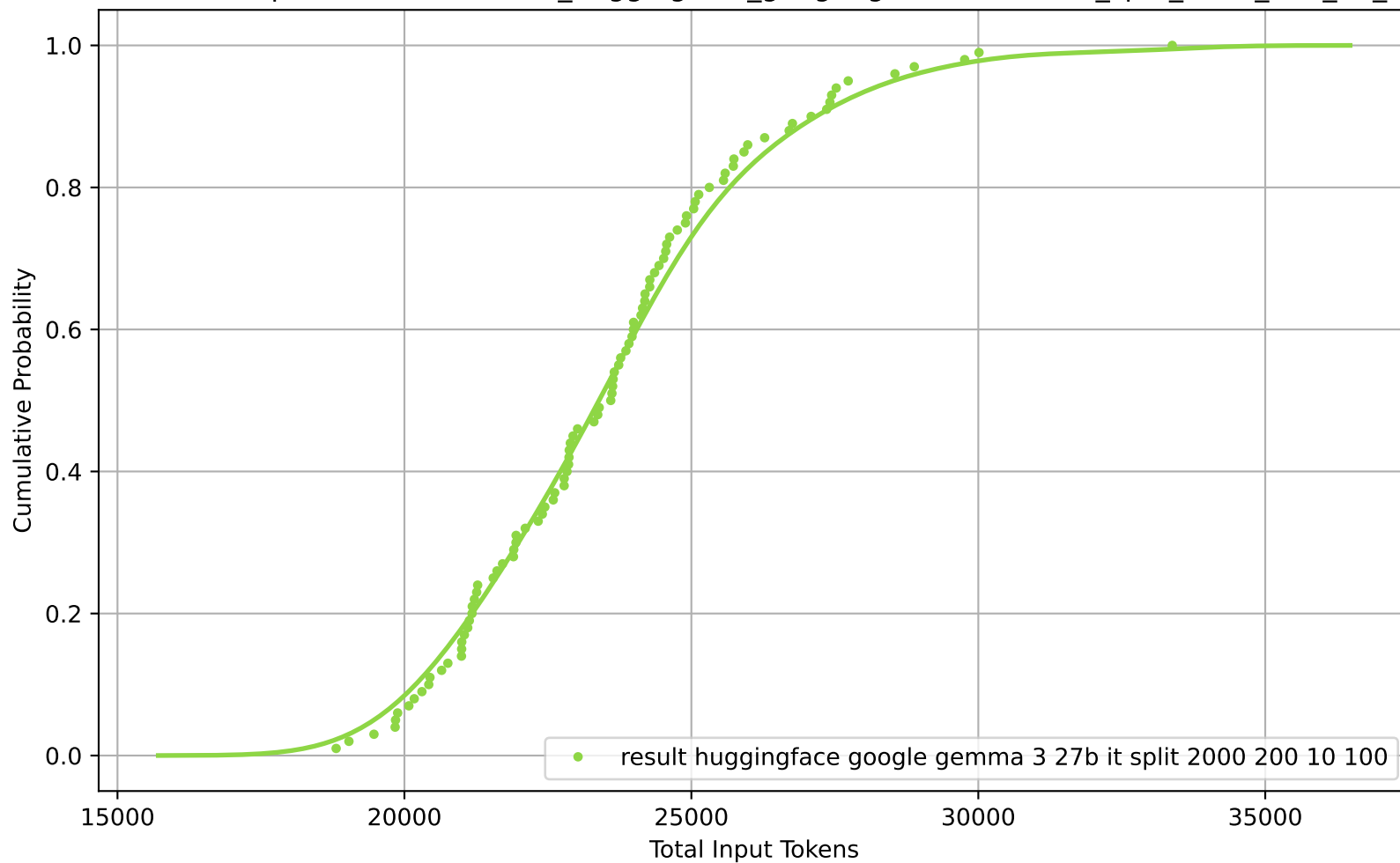
CDF of Total Input Tokens for result_huggingface_google-gemma-3-27b-it_split_2000_200_10_100
