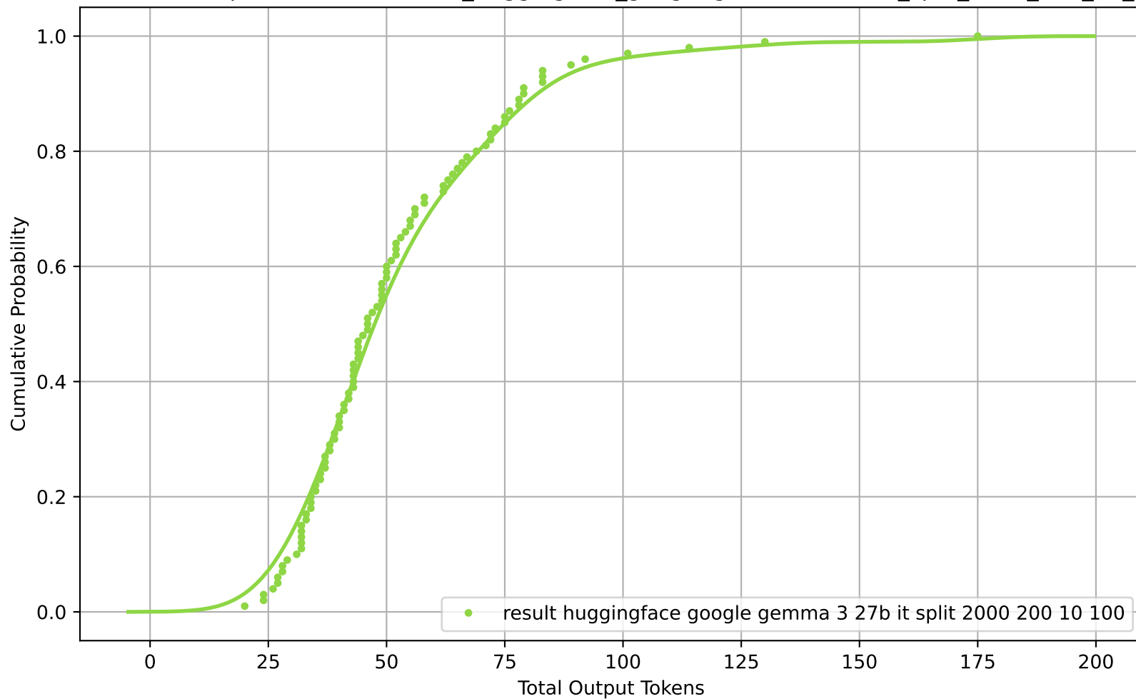
CDF of Total Output Tokens for result_huggingface_google-gemma-3-27b-it_split_2000_200_10_100
