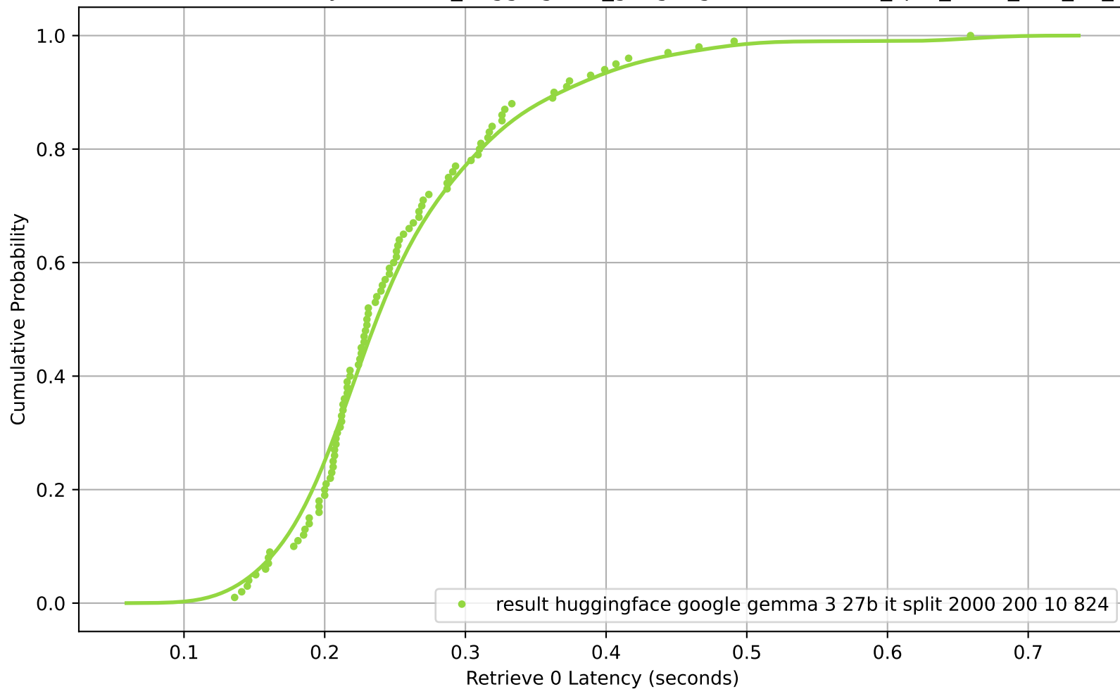
CDF of Retrieve 0 Latency for result_huggingface_google-gemma-3-27b-it_split_2000_200_10_824
