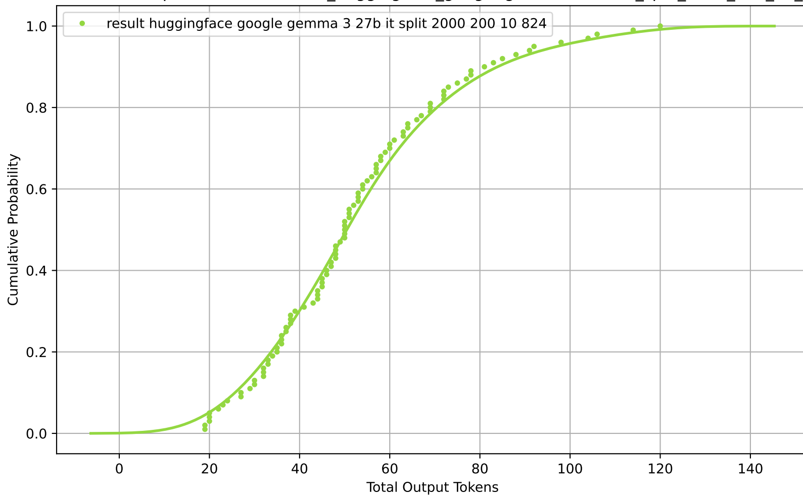
CDF of Total Output Tokens for result_huggingface_google-gemma-3-27b-it_split_2000_200_10_824
