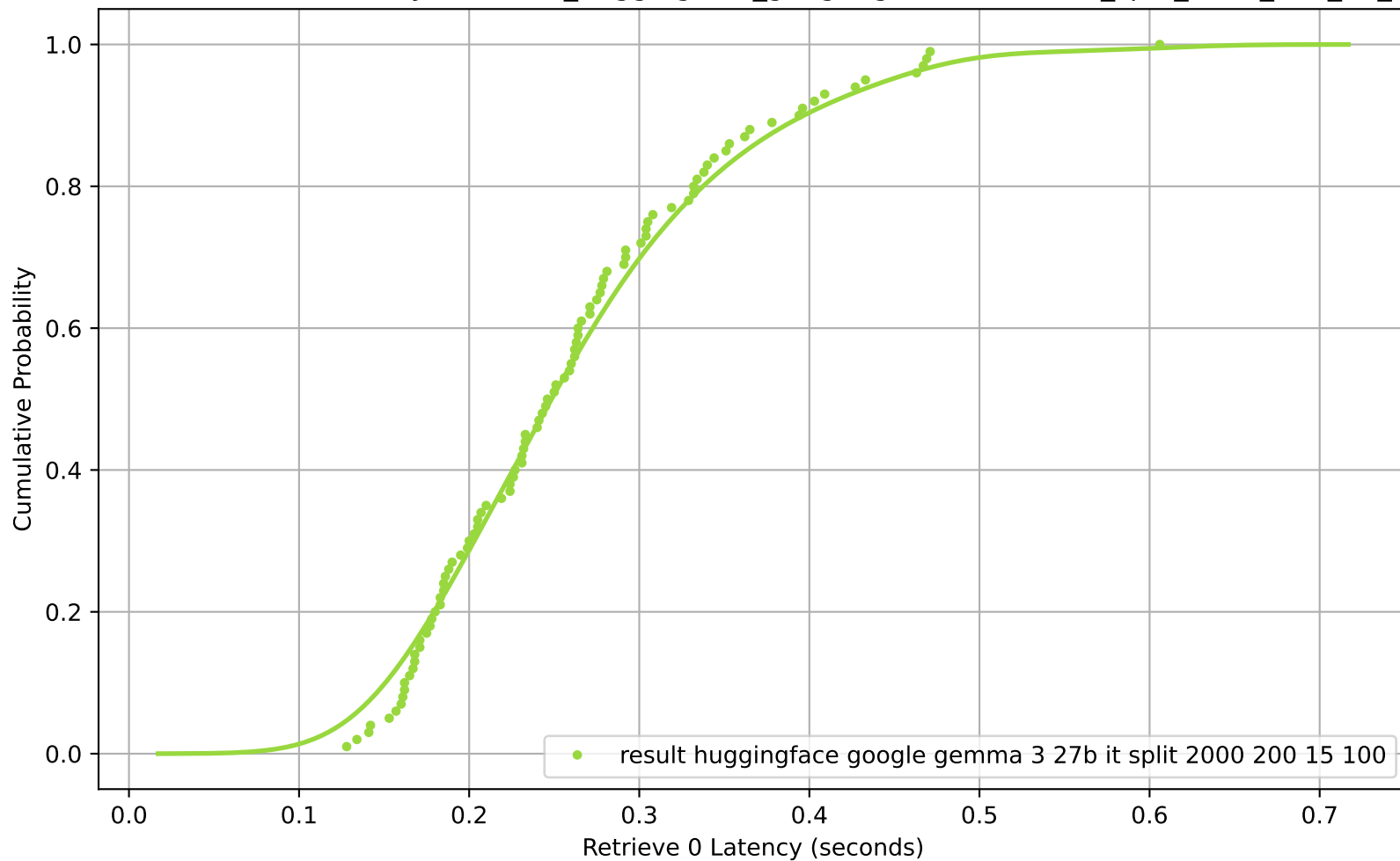
CDF of Retrieve 0 Latency for result_huggingface_google-gemma-3-27b-it_split_2000_200_15_100
