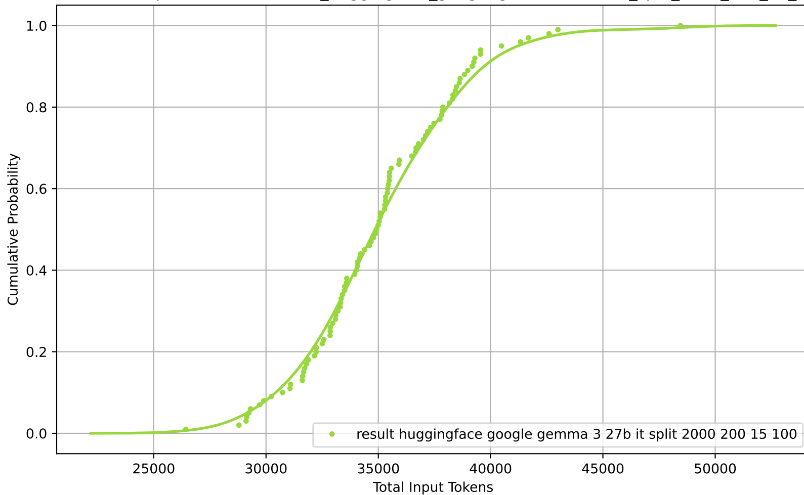
CDF of Total Input Tokens for result_huggingface_google-gemma-3-27b-it_split_2000_200_15_100
