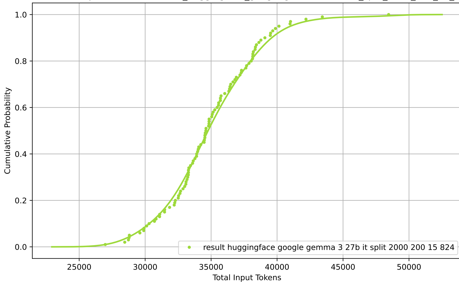
CDF of Total Input Tokens for result_huggingface_google-gemma-3-27b-it_split_2000_200_15_824
