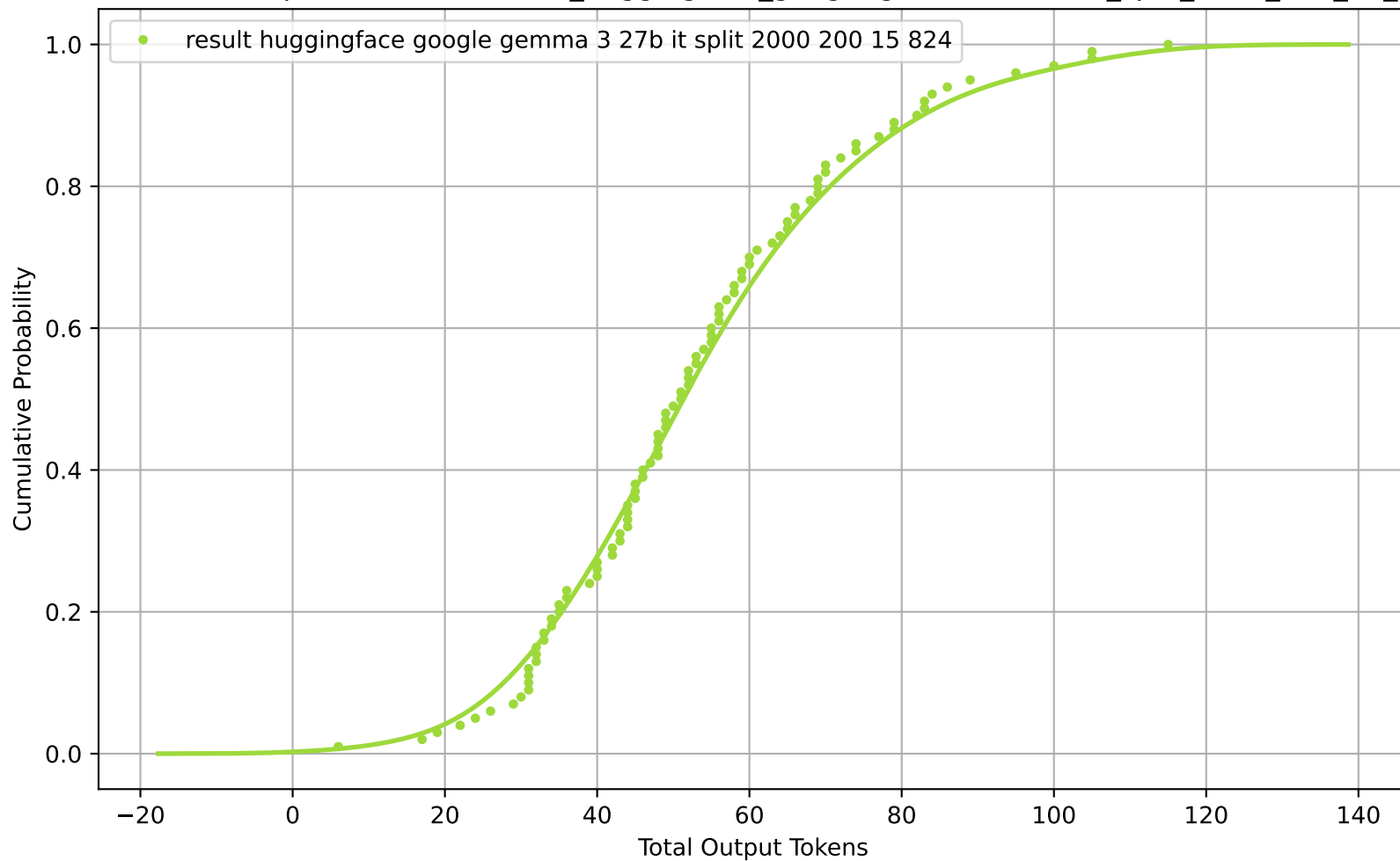
CDF of Total Output Tokens for result_huggingface_google-gemma-3-27b-it_split_2000_200_15_824
