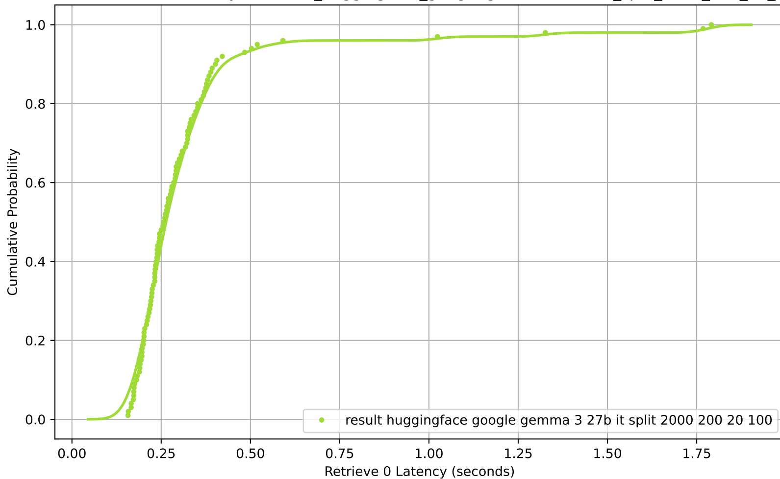
CDF of Retrieve 0 Latency for result_huggingface_google-gemma-3-27b-it_split_2000_200_20_100
