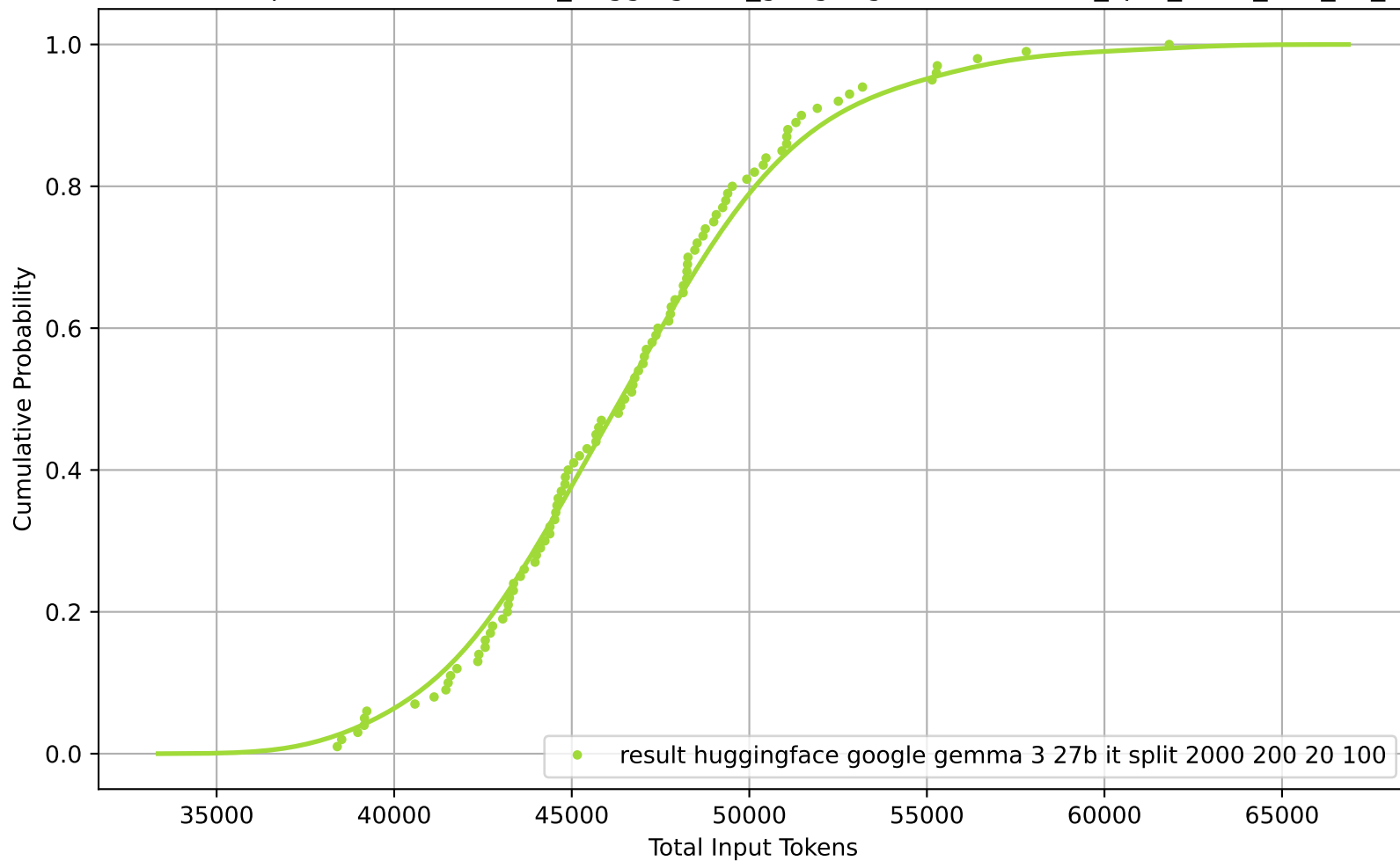
CDF of Total Input Tokens for result_huggingface_google-gemma-3-27b-it_split_2000_200_20_100
