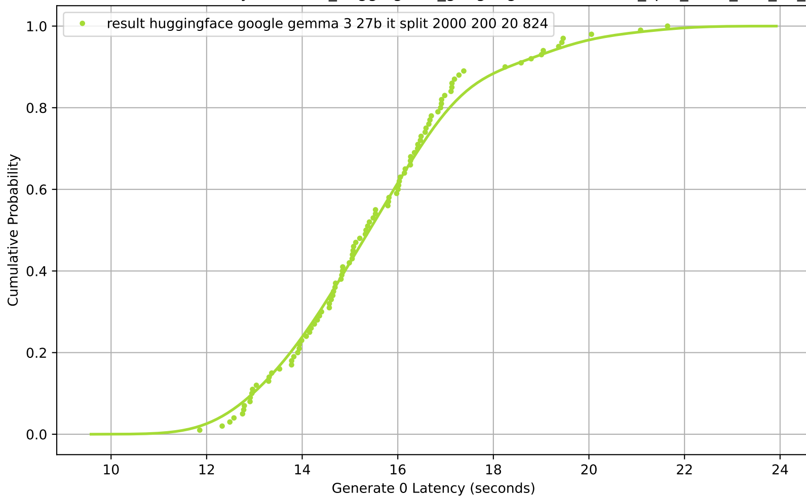
CDF of Generate 0 Latency for result_huggingface_google-gemma-3-27b-it_split_2000_200_20_824
