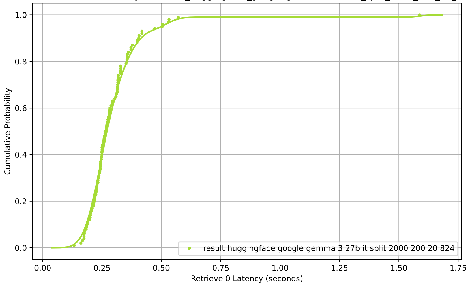
CDF of Retrieve 0 Latency for result_huggingface_google-gemma-3-27b-it_split_2000_200_20_824
