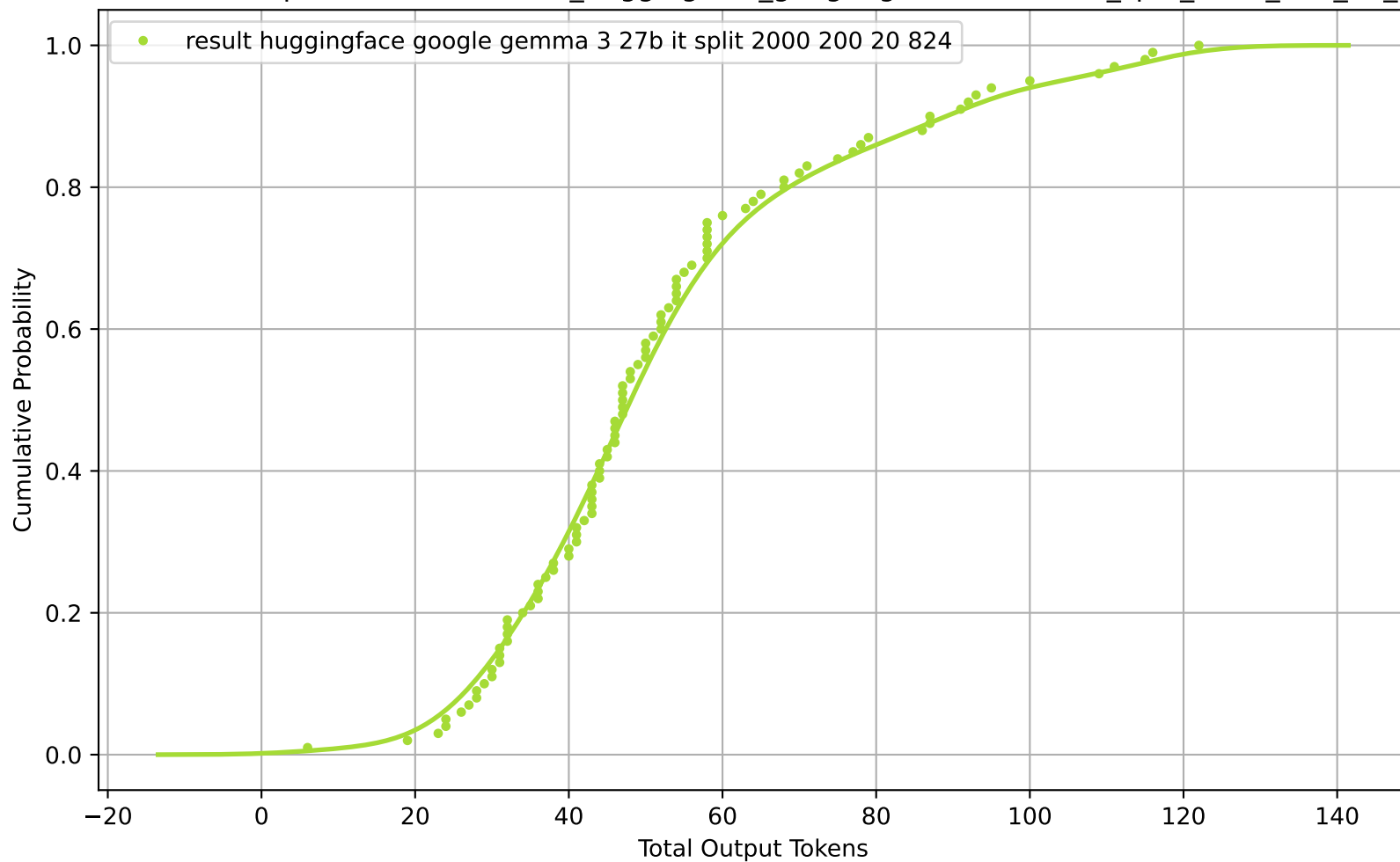
CDF of Total Output Tokens for result_huggingface_google-gemma-3-27b-it_split_2000_200_20_824
