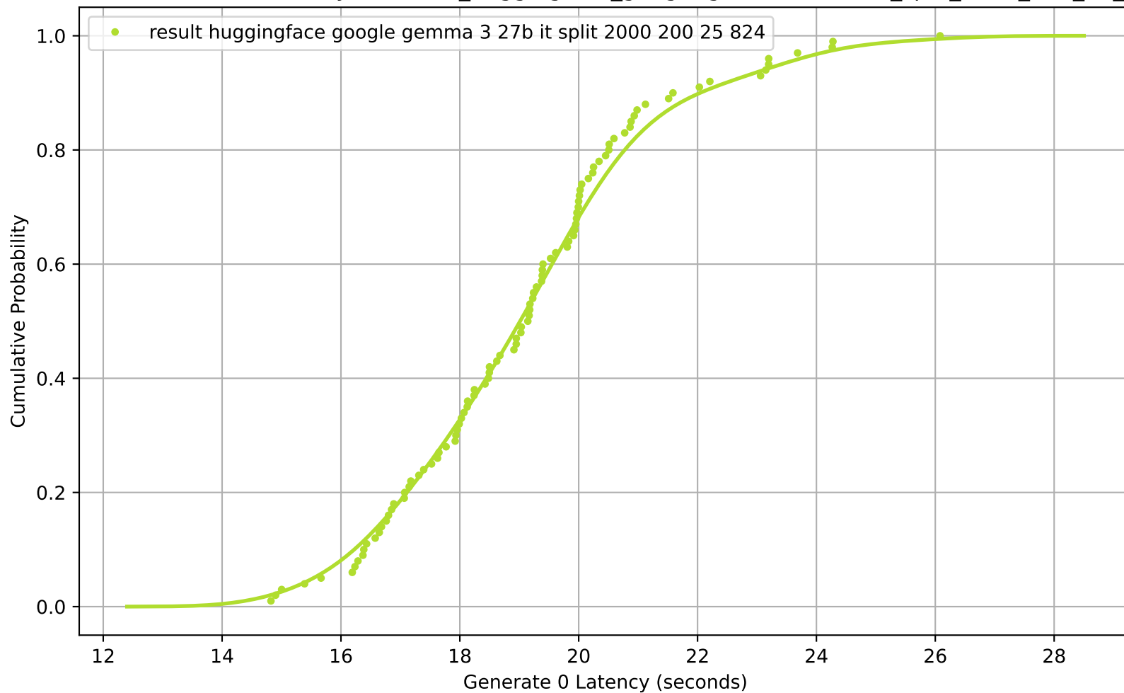
CDF of Generate 0 Latency for result_huggingface_google-gemma-3-27b-it_split_2000_200_25_824
