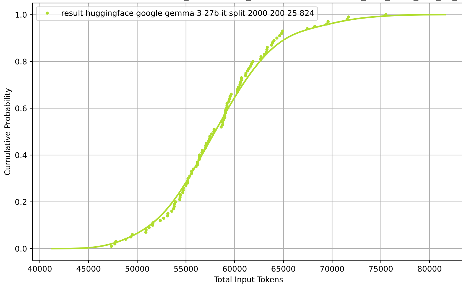
CDF of Total Input Tokens for result_huggingface_google-gemma-3-27b-it_split_2000_200_25_824
