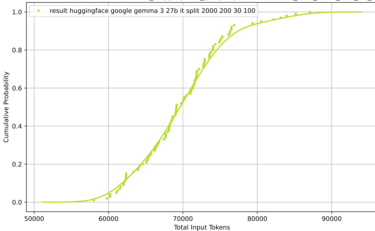
CDF of Total Input Tokens for result_huggingface_google-gemma-3-27b-it_split_2000_200_30_100
