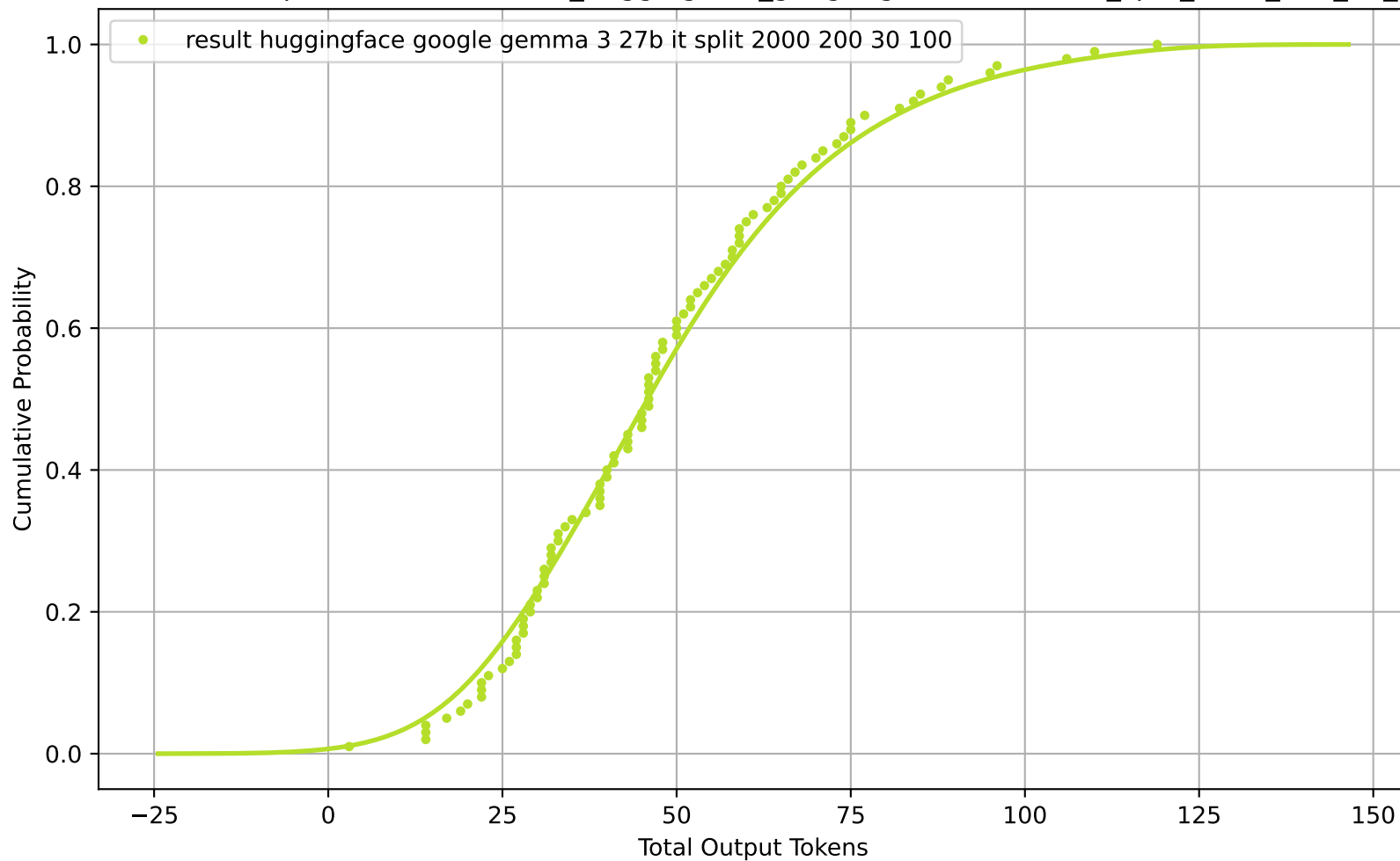
CDF of Total Output Tokens for result_huggingface_google-gemma-3-27b-it_split_2000_200_30_100
