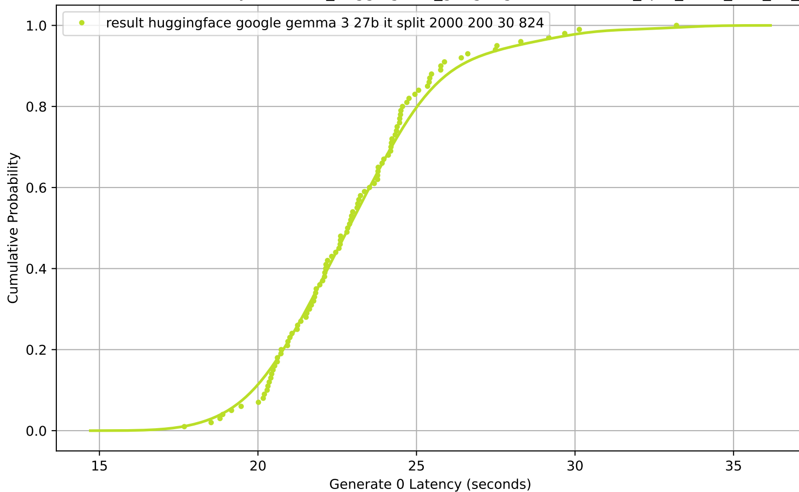
CDF of Generate 0 Latency for result_huggingface_google-gemma-3-27b-it_split_2000_200_30_824
