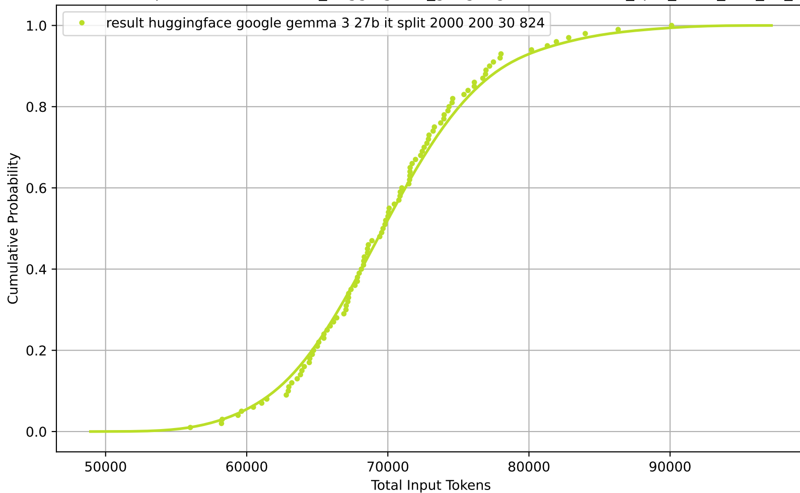
CDF of Total Input Tokens for result_huggingface_google-gemma-3-27b-it_split_2000_200_30_824
