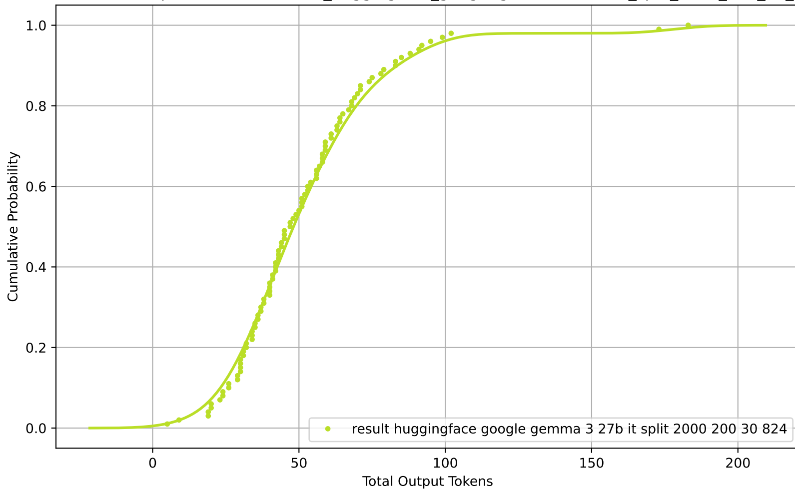
CDF of Total Output Tokens for result_huggingface_google-gemma-3-27b-it_split_2000_200_30_824
