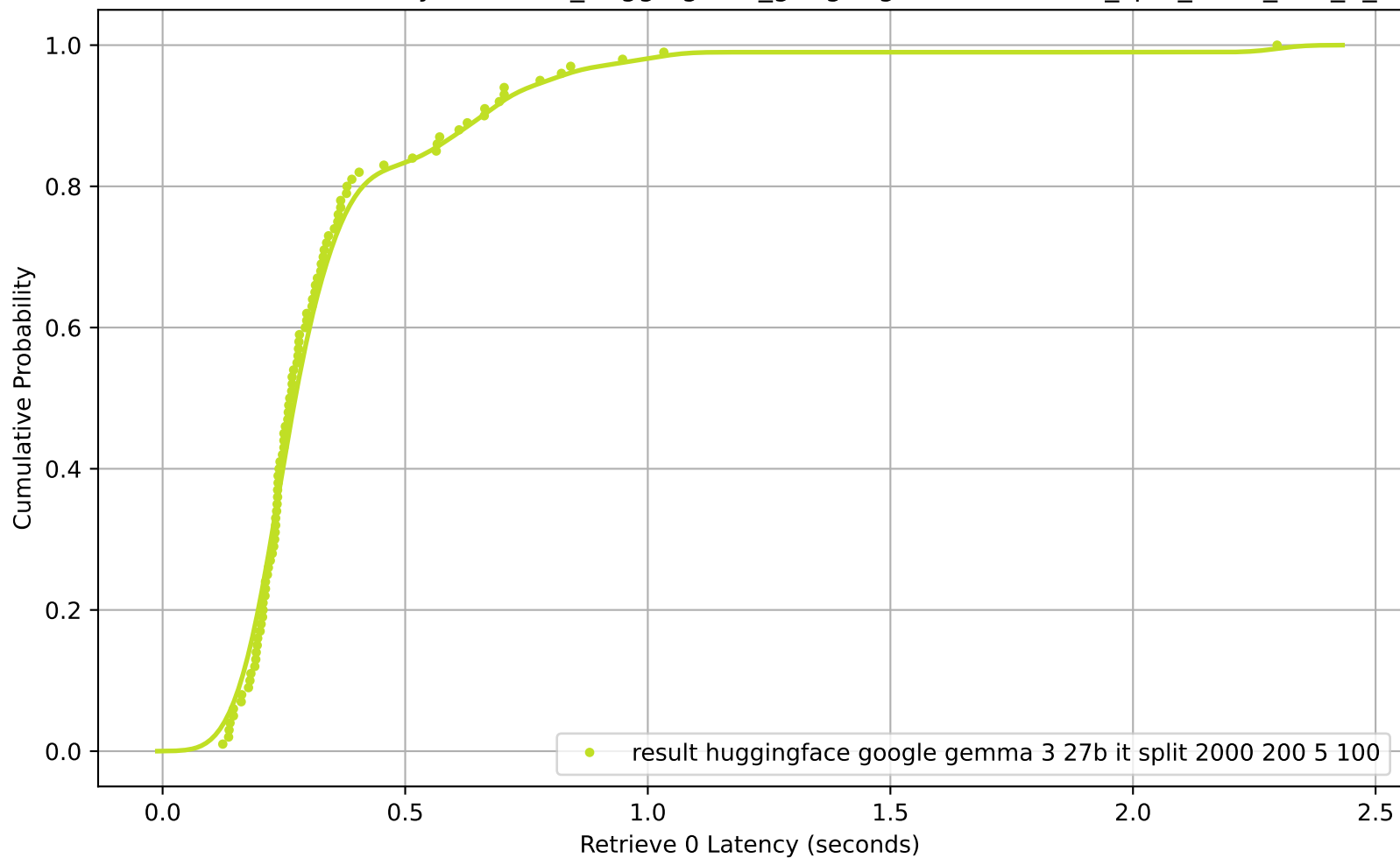
CDF of Retrieve 0 Latency for result_huggingface_google-gemma-3-27b-it_split_2000_200_5_100
