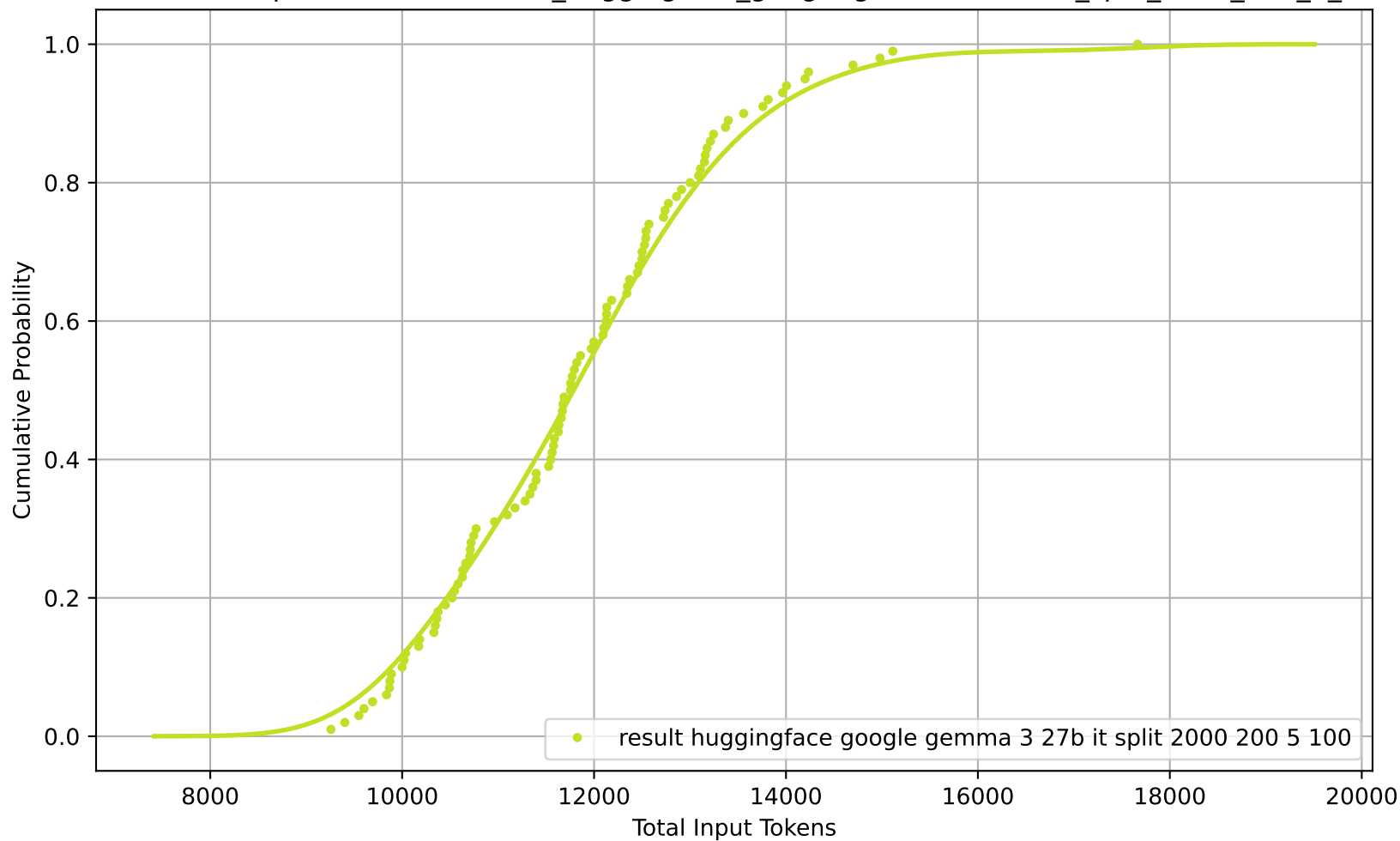
CDF of Total Input Tokens for result_huggingface_google-gemma-3-27b-it_split_2000_200_5_100
