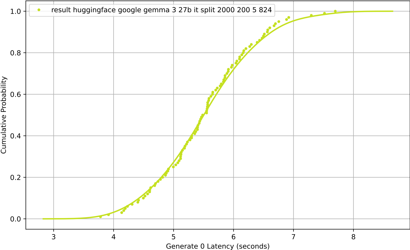
CDF of Generate 0 Latency for result_huggingface_google-gemma-3-27b-it_split_2000_200_5_824
