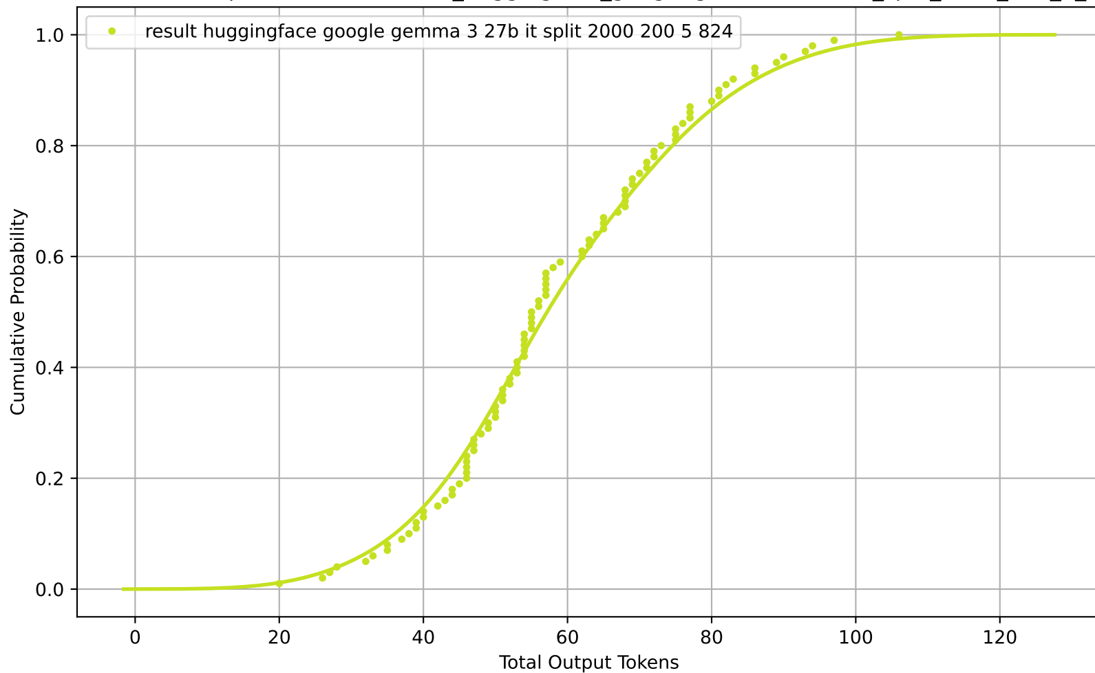
CDF of Total Output Tokens for result_huggingface_google-gemma-3-27b-it_split_2000_200_5_824
