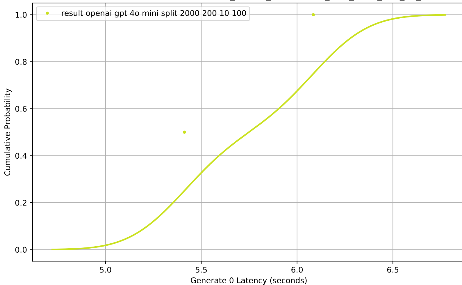
CDF of Generate 0 Latency for result_openai_gpt-4o-mini_split_2000_200_10_100
