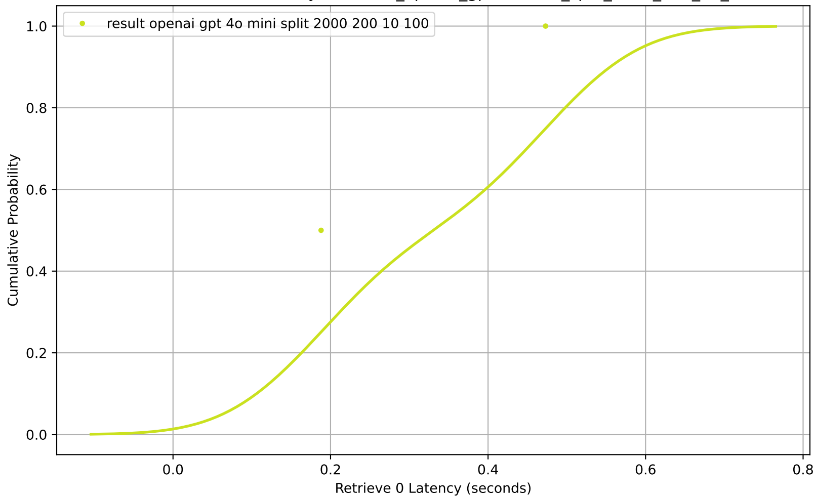
CDF of Retrieve 0 Latency for result_openai_gpt-4o-mini_split_2000_200_10_100
