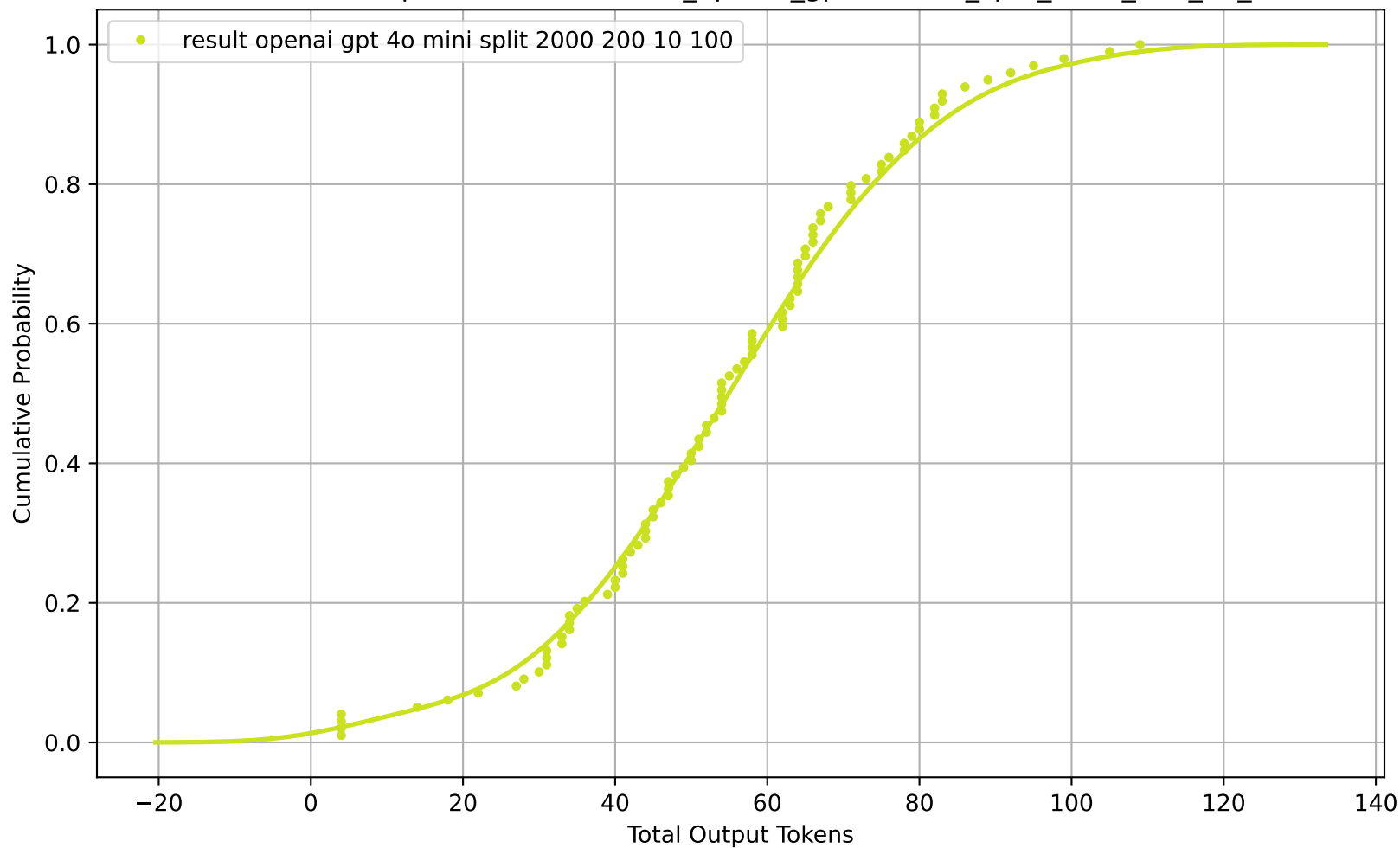
CDF of Total Output Tokens for result_openai_gpt-4o-mini_split_2000_200_10_100
