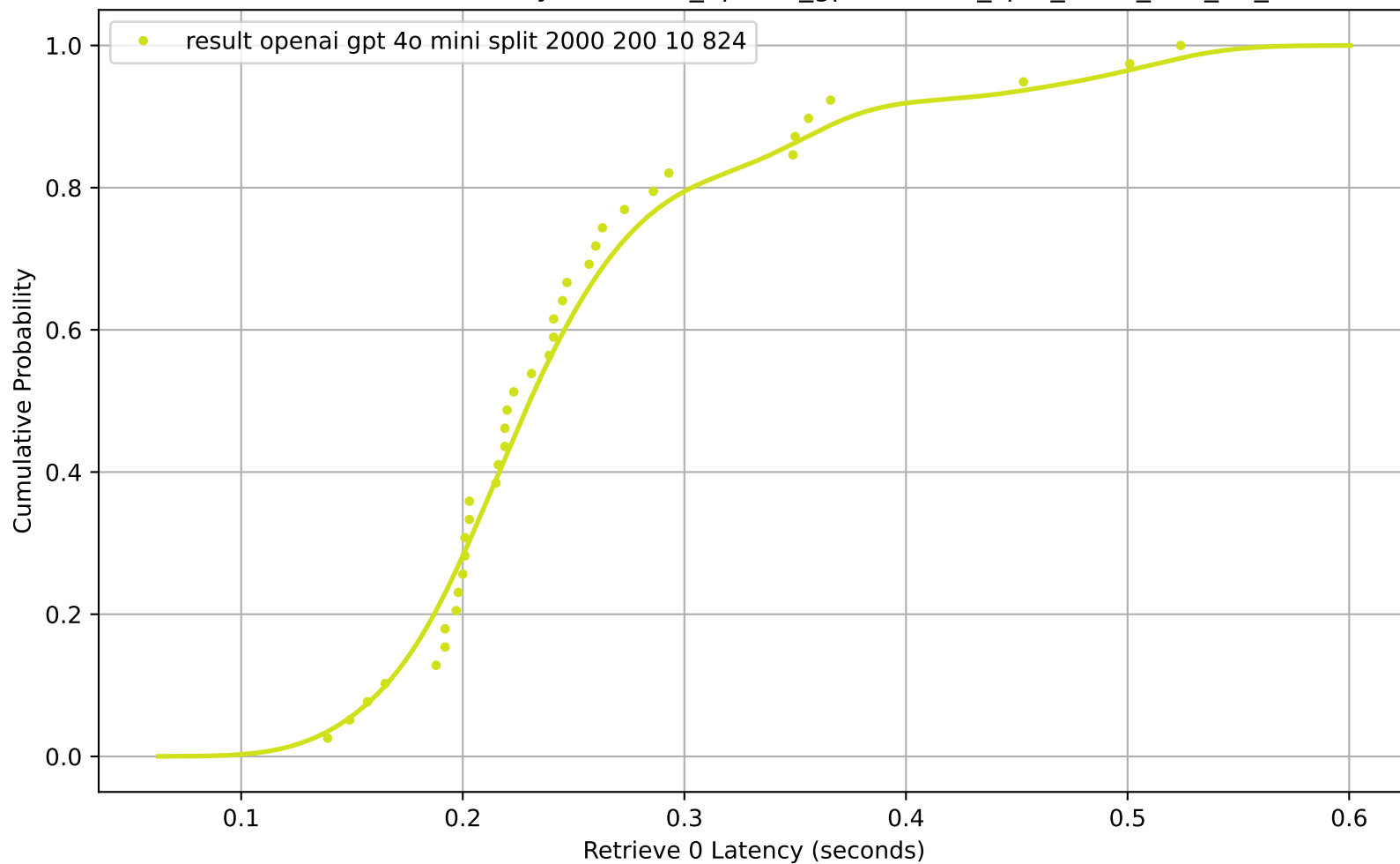
CDF of Retrieve 0 Latency for result_openai_gpt-4o-mini_split_2000_200_10_824
