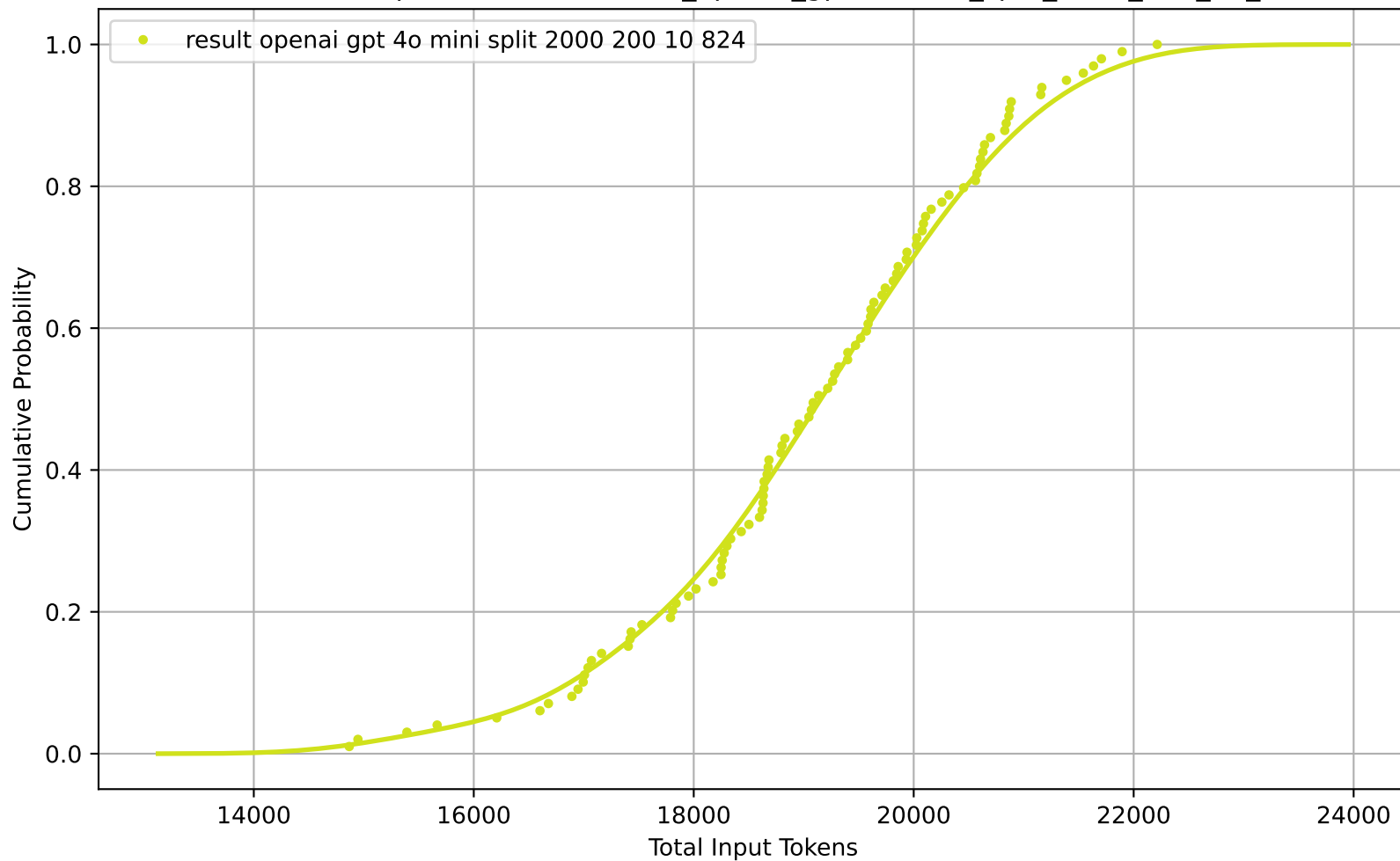
CDF of Total Input Tokens for result_openai_gpt-4o-mini_split_2000_200_10_824
