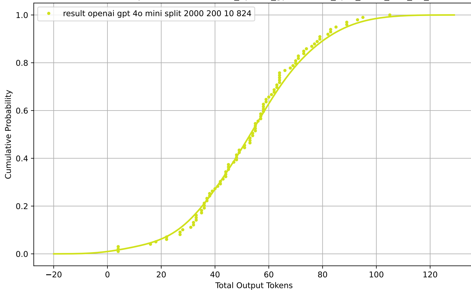
CDF of Total Output Tokens for result_openai_gpt-4o-mini_split_2000_200_10_824
