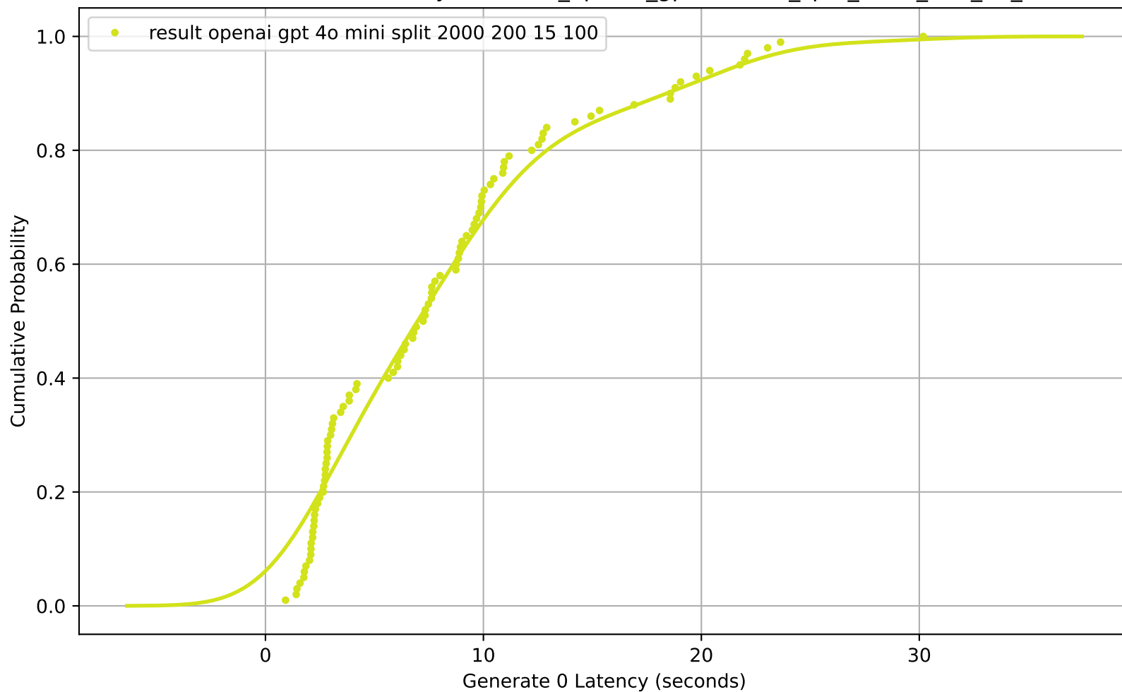
CDF of Generate 0 Latency for result_openai_gpt-4o-mini_split_2000_200_15_100
