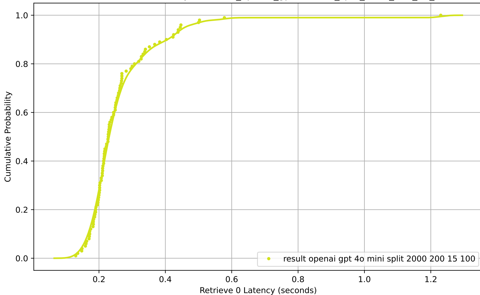
CDF of Retrieve 0 Latency for result_openai_gpt-4o-mini_split_2000_200_15_100
