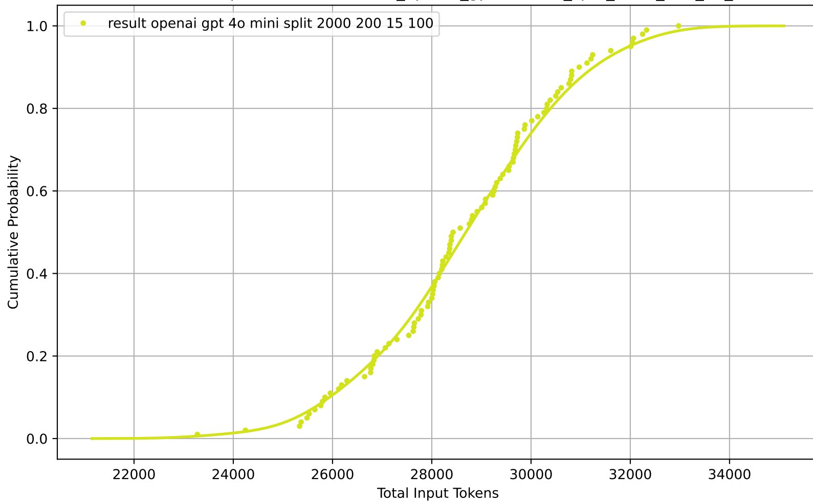
CDF of Total Input Tokens for result_openai_gpt-4o-mini_split_2000_200_15_100
