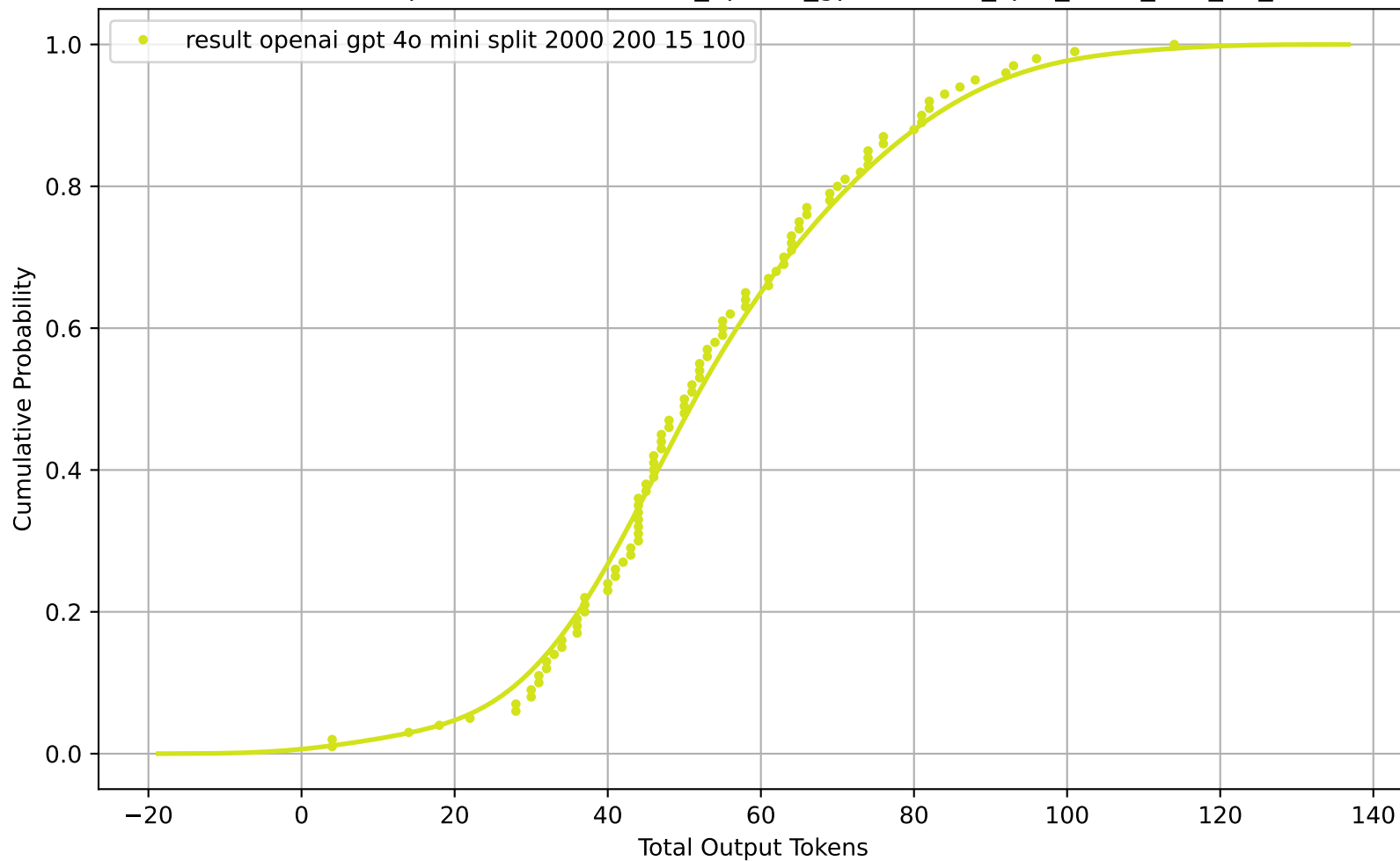
CDF of Total Output Tokens for result_openai_gpt-4o-mini_split_2000_200_15_100
