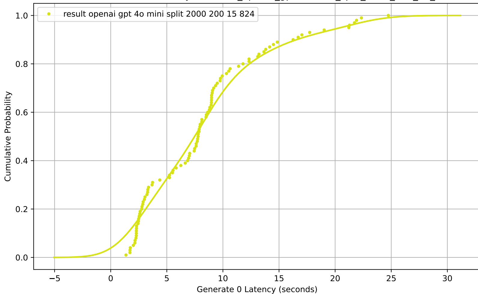
CDF of Generate 0 Latency for result_openai_gpt-4o-mini_split_2000_200_15_824
