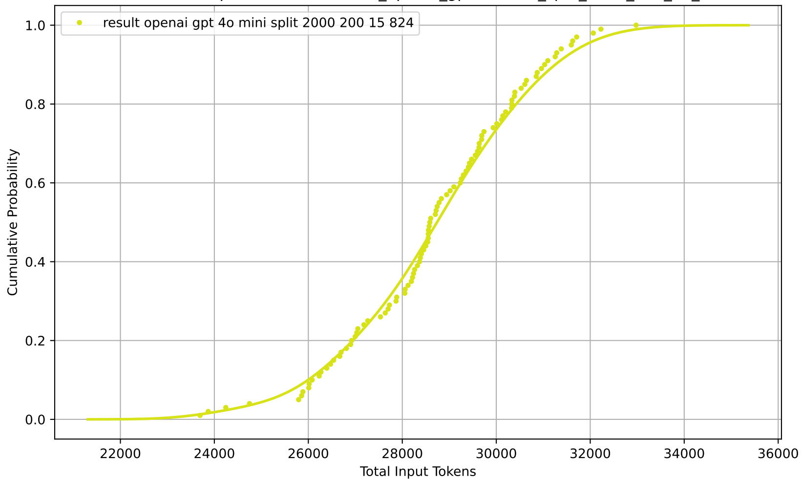
CDF of Total Input Tokens for result_openai_gpt-4o-mini_split_2000_200_15_824
