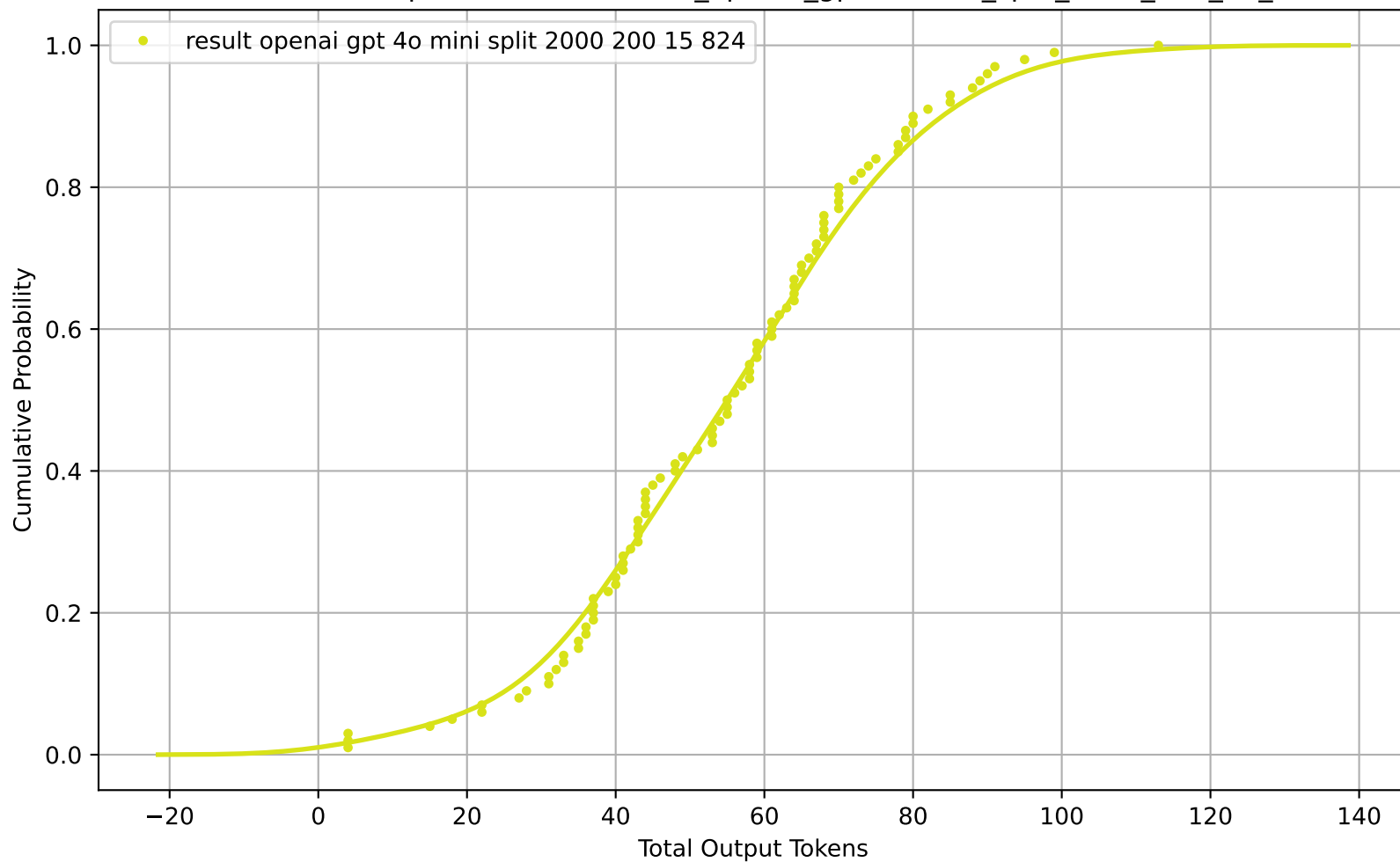
CDF of Total Output Tokens for result_openai_gpt-4o-mini_split_2000_200_15_824
