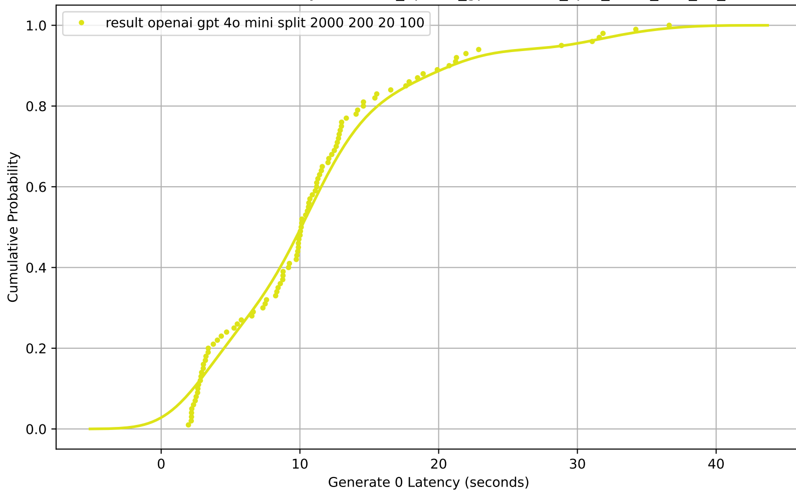
CDF of Generate 0 Latency for result_openai_gpt-4o-mini_split_2000_200_20_100
