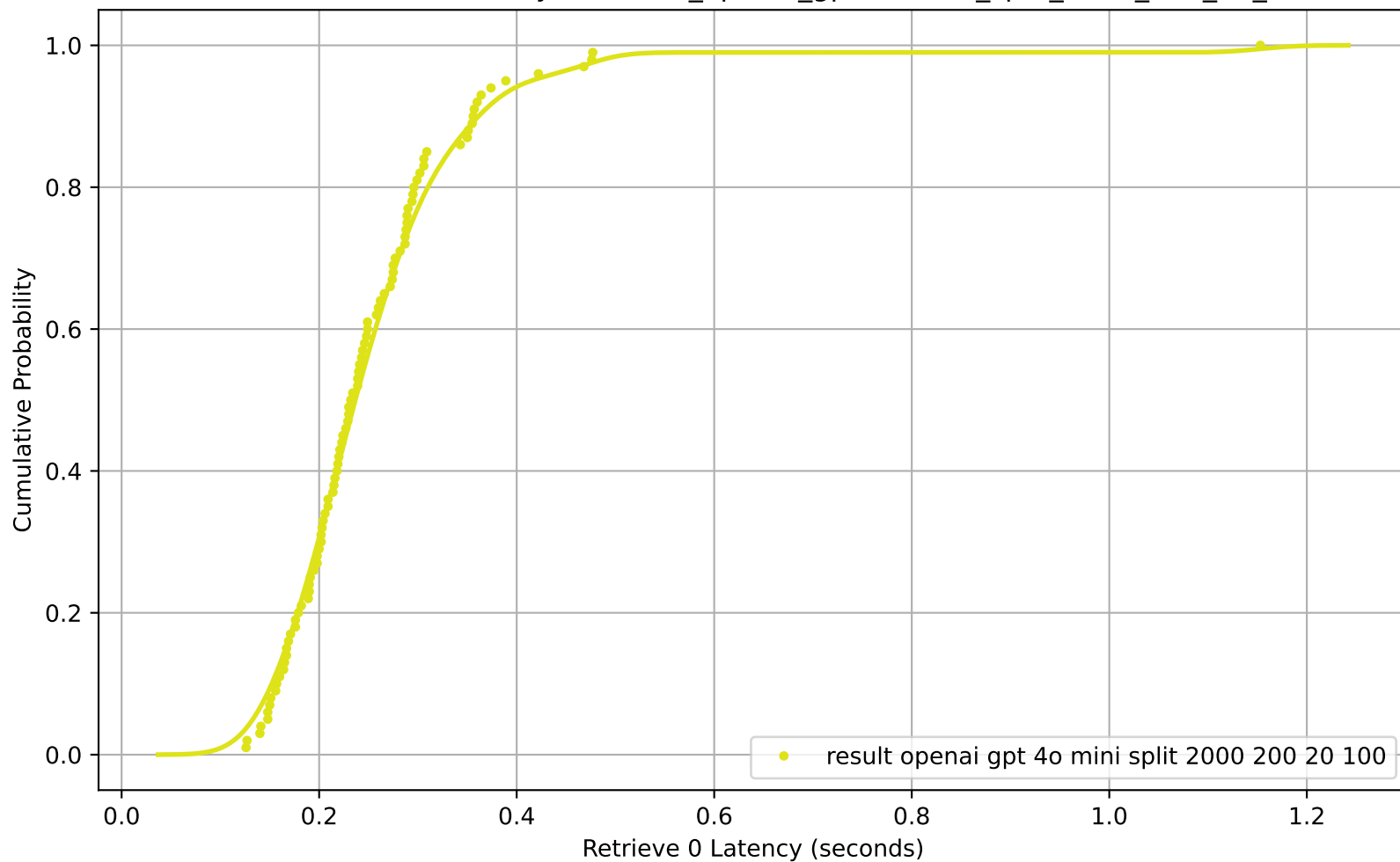
CDF of Retrieve 0 Latency for result_openai_gpt-4o-mini_split_2000_200_20_100
