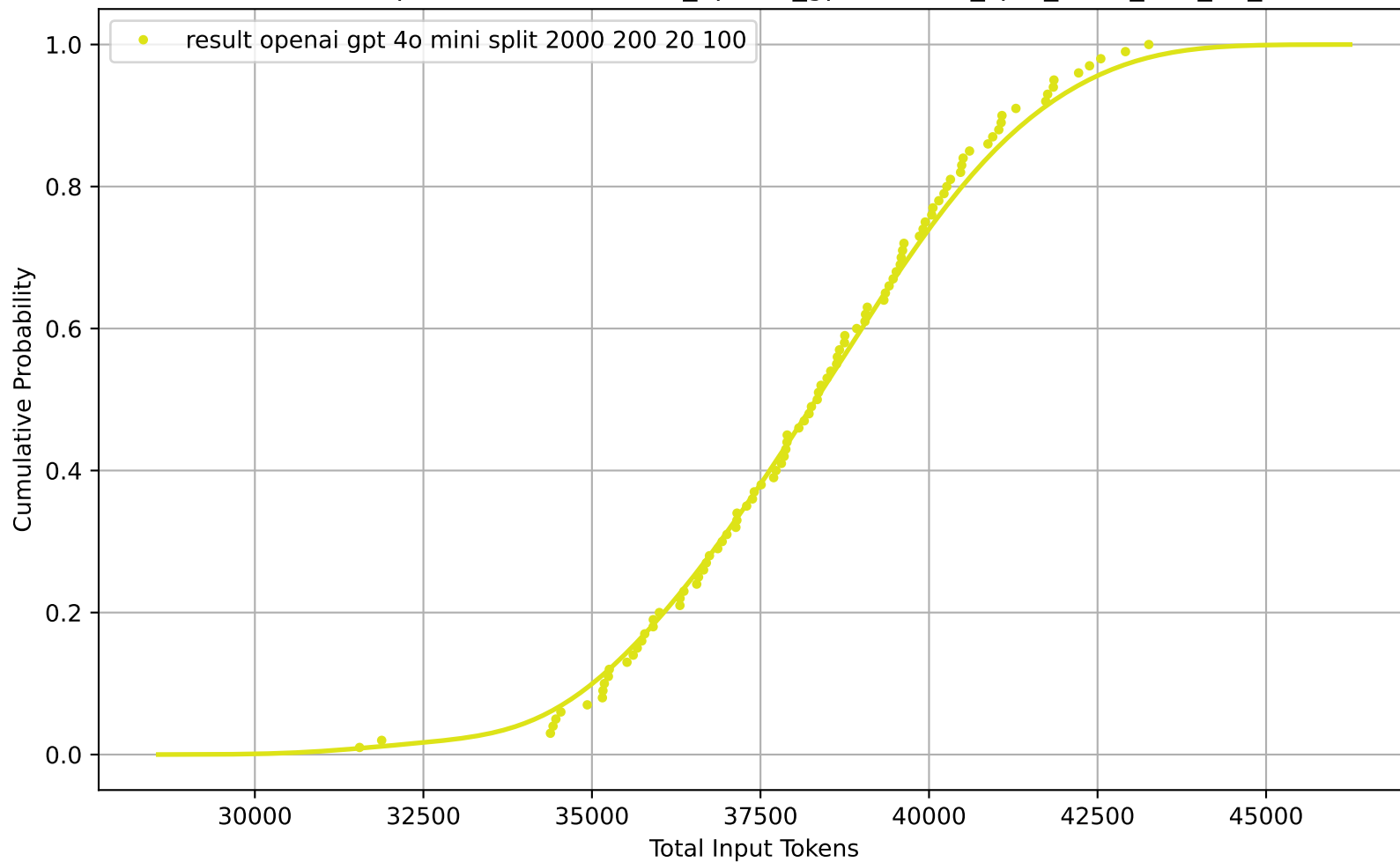
CDF of Total Input Tokens for result_openai_gpt-4o-mini_split_2000_200_20_100
