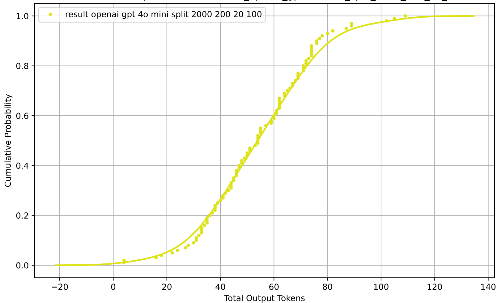
CDF of Total Output Tokens for result_openai_gpt-4o-mini_split_2000_200_20_100
