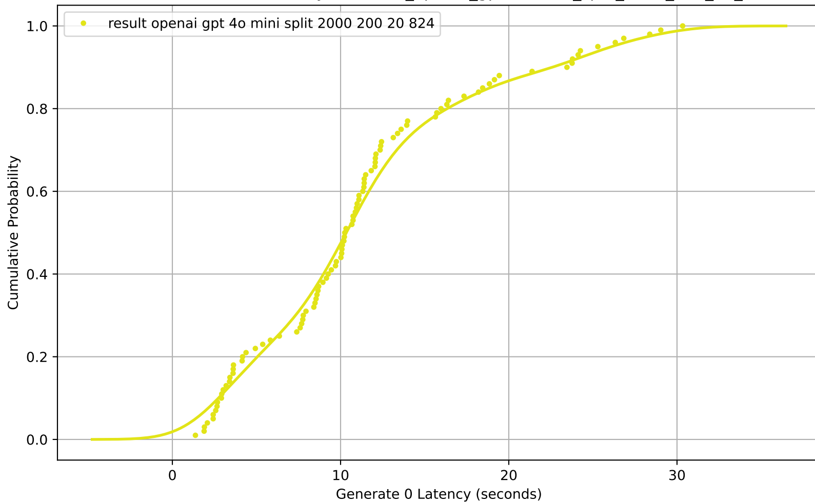
CDF of Generate 0 Latency for result_openai_gpt-4o-mini_split_2000_200_20_824
