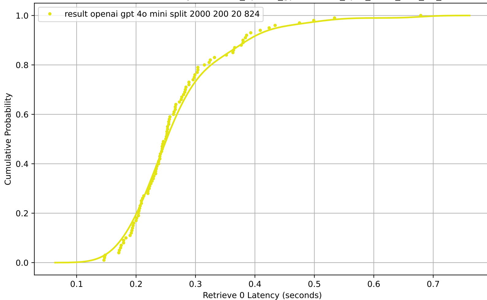
CDF of Retrieve 0 Latency for result_openai_gpt-4o-mini_split_2000_200_20_824
